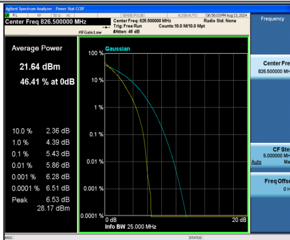
Band5-5MHz-QPSK-20425-25RB#0-PASS
