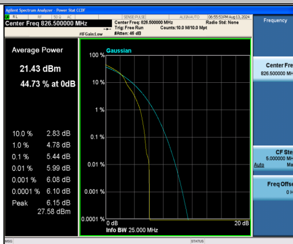
Band5-5MHz-16QAM-20425-1RB#0-PASS
