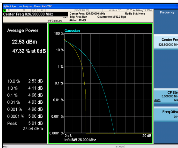
Band5-5MHz-QPSK-20425-1RB#0-PASS
