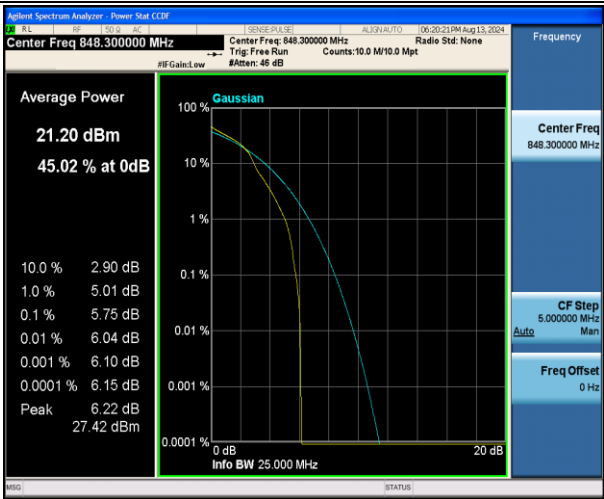
Band5-1.4MHz-16QAM-20643-1RB#0-PASS
