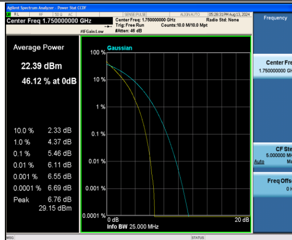
Band4-10MHz-QPSK-20350-50RB#0-PASS
