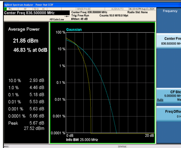
Band5-1.4MHz-16QAM-20525-1RB#0-PASS
