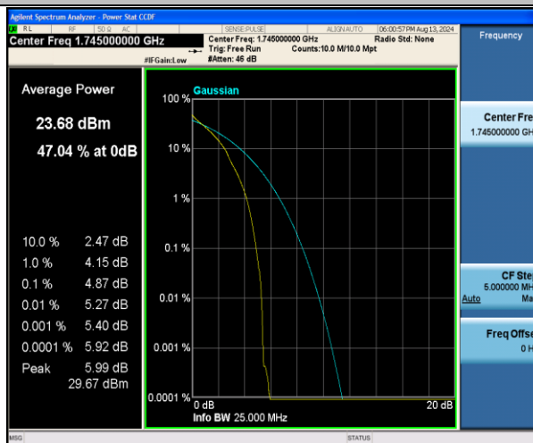
Band4-20MHz-QPSK-20300-1RB#0-PASS
