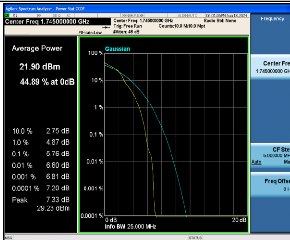
Band4-20MHz-16QAM-20300-1RB#0-PASS
