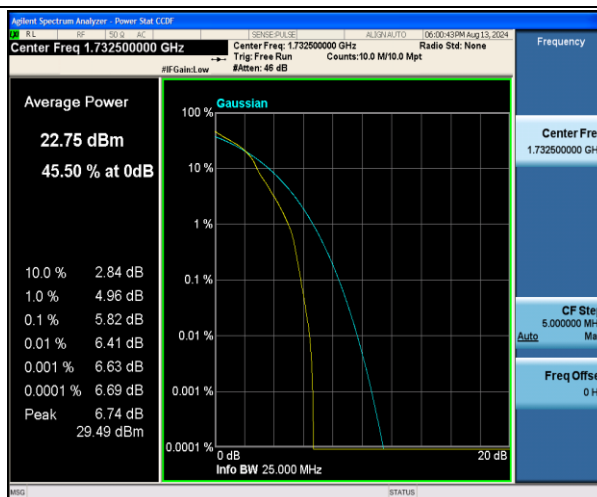
Band4-20MHz-16QAM-20175-1RB#0-PASS
