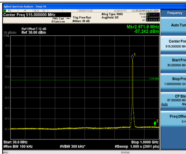
Band5-4132-30~1000MHz-PASS
