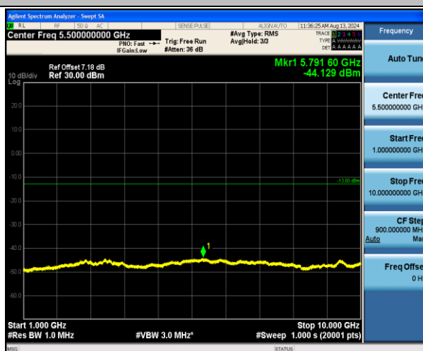
Band5-4233-1000~10000MHz-PASS
