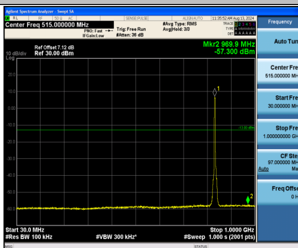
Band5-4182-30~1000MHz-PASS
