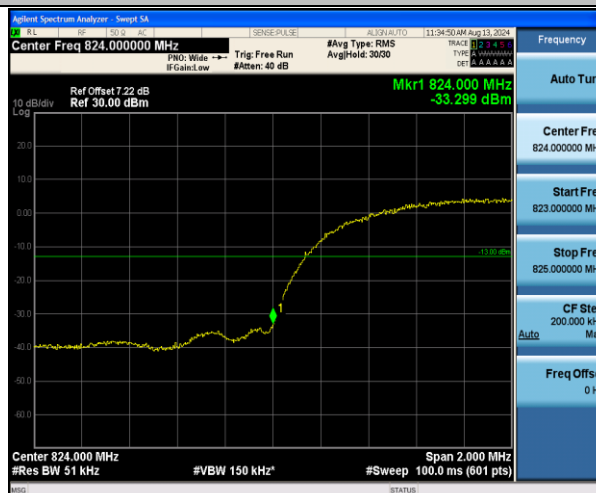
Band5-4132-PASS
