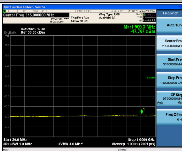
Band2-9538-30~1000MHz-PASS
