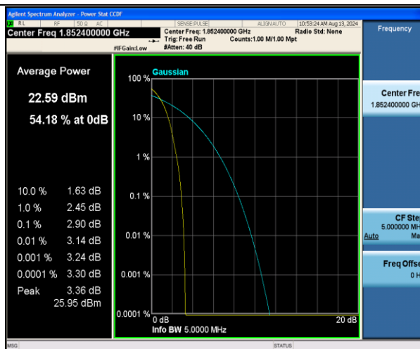
Band2-9262-PASS
