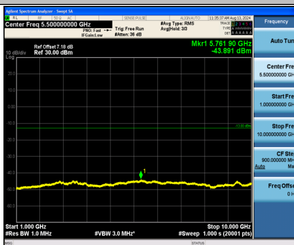
Band5-4132-1000~10000MHz-PASS
