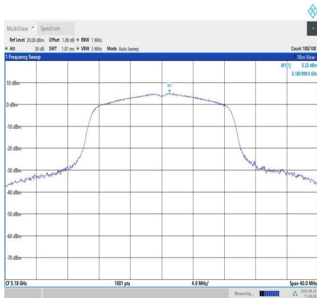
11N20SISO-Ant1-5180-PASS
