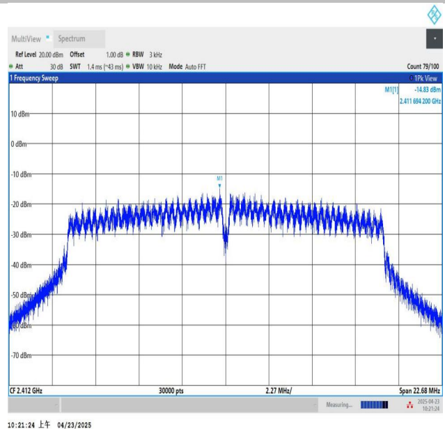
11G-Ant1-2412-PASS
