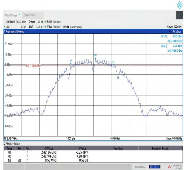
11B-Ant1-2437-PASS
