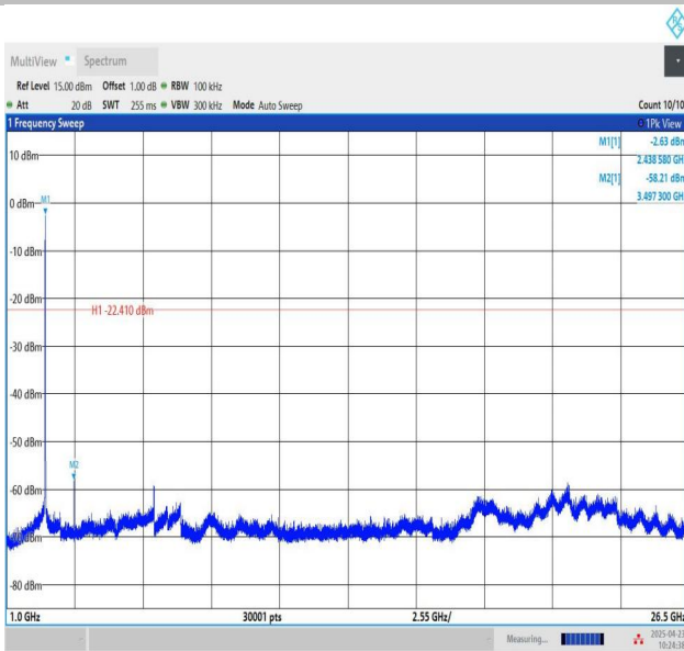
11G-Ant1-2437-0~Reference-PASS
