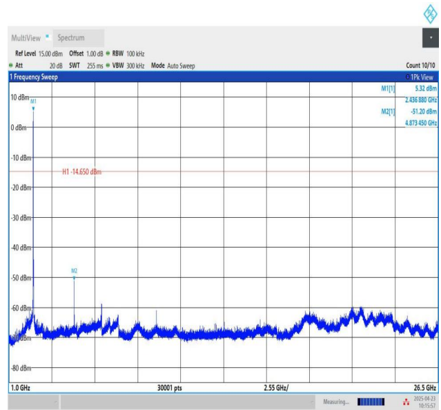
11B-Ant1-2437-1000~26500-PASS
