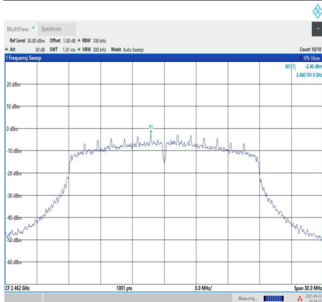
11N20SISO-Ant1-2462-0~Reference-PASS
