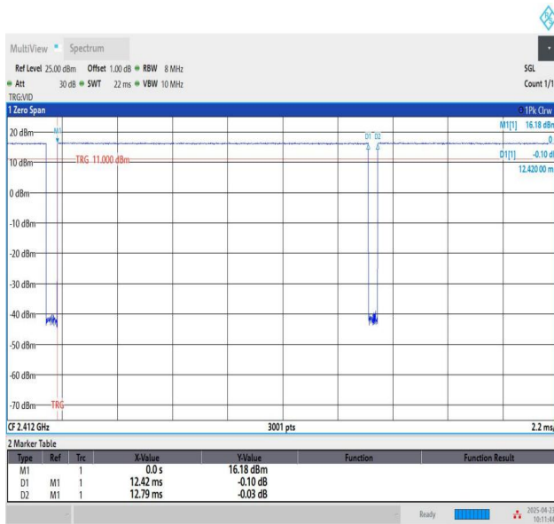
NTNV-11B-Ant1-2412
