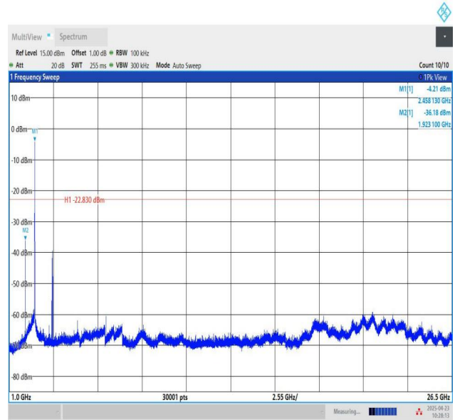
11G-Ant1-2462-1000~26500-PASS
