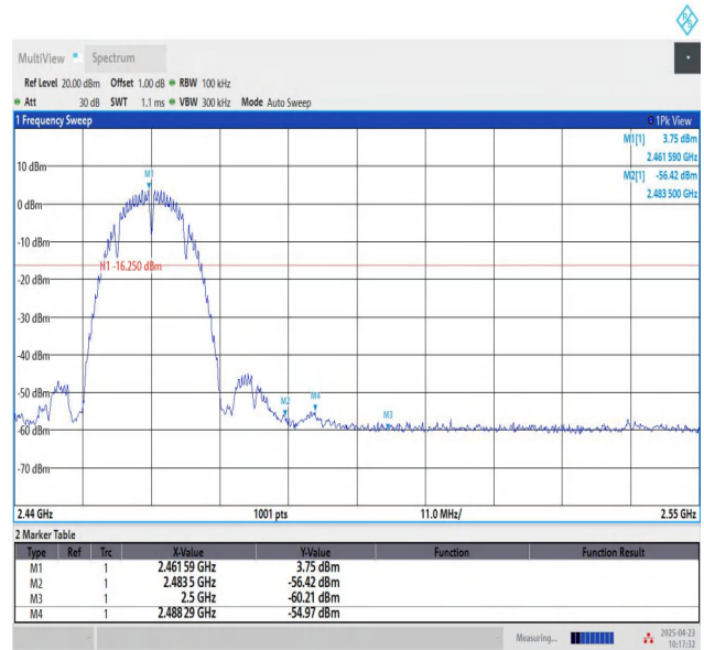
11B-Ant1-2462-PASS
