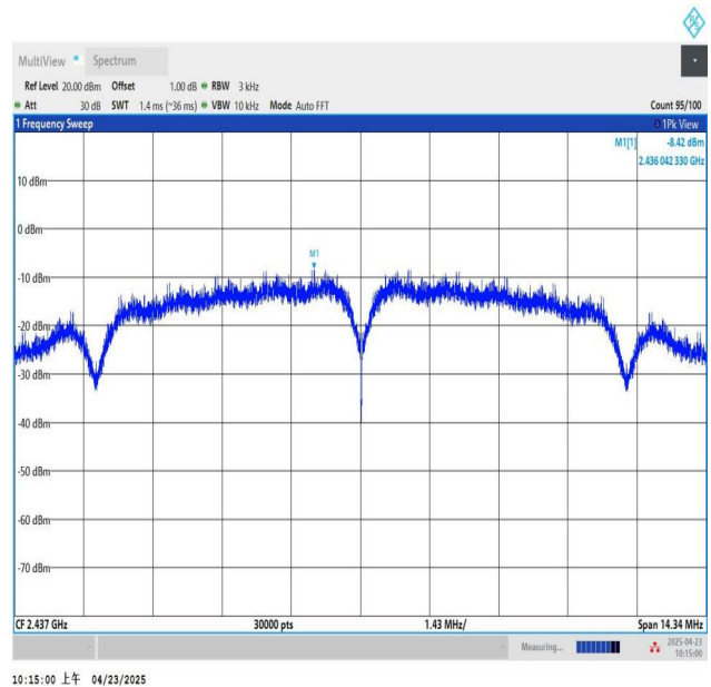
11B-Ant1-2437-PASS
