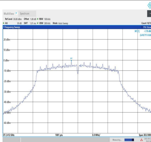
11G-Ant1-2412-0~Reference-PASS
