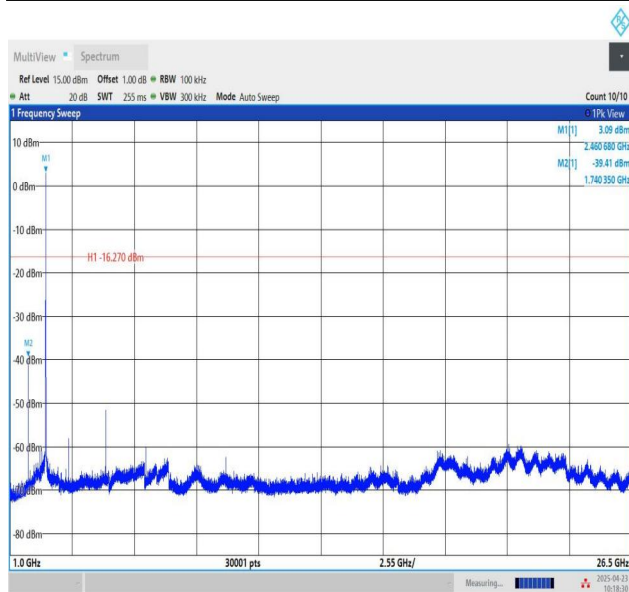
11B-Ant1-2462-1000~26500-PASS
