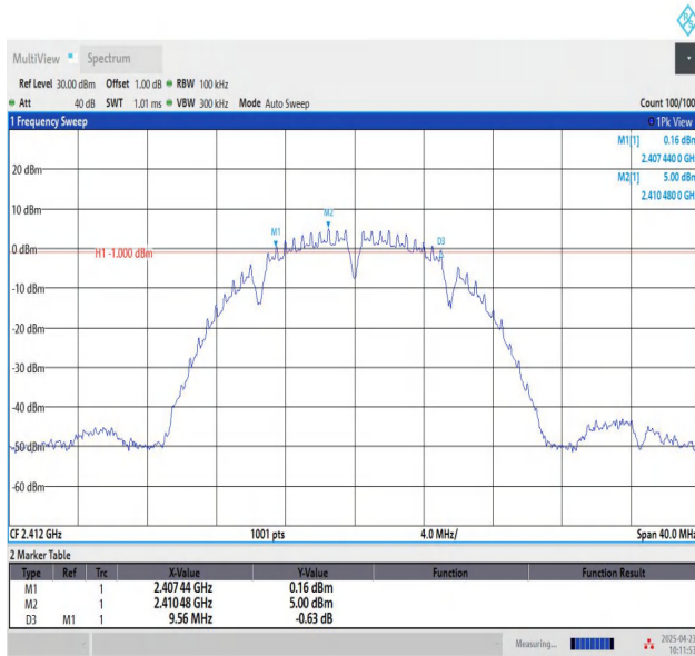
11B-Ant1-2412-PASS
