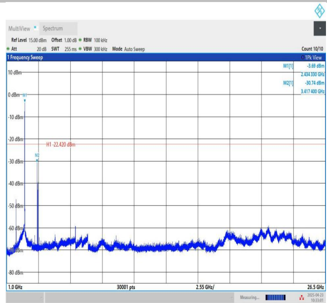
11N20SISO-Ant1-2437-0~Reference-PASS
