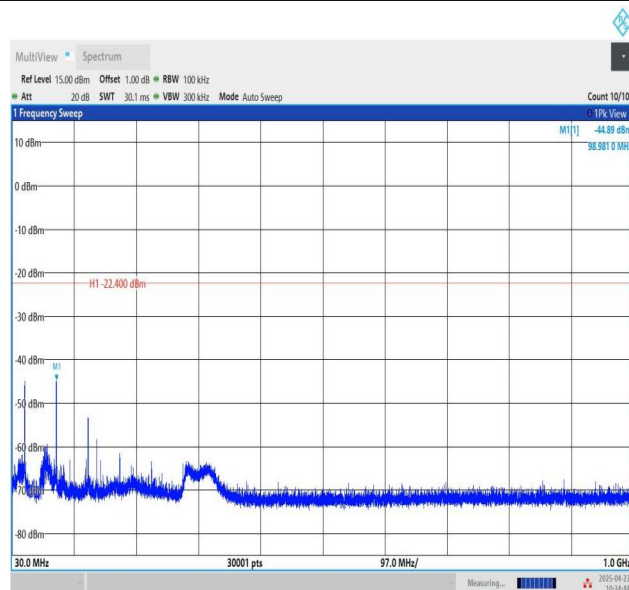
11N20SISO-Ant1-2462-30~1000-PASS
