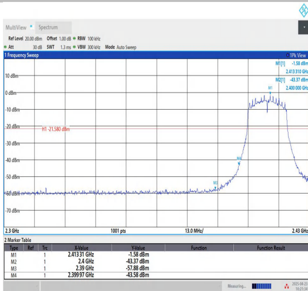
11B-Ant1-2412-PASS
