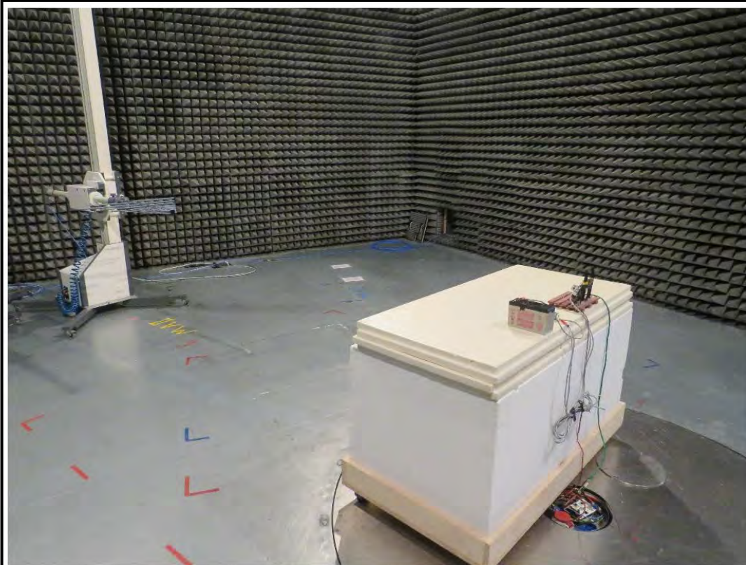
TEST SETUP Radiated emissions 0.2-1GHz
