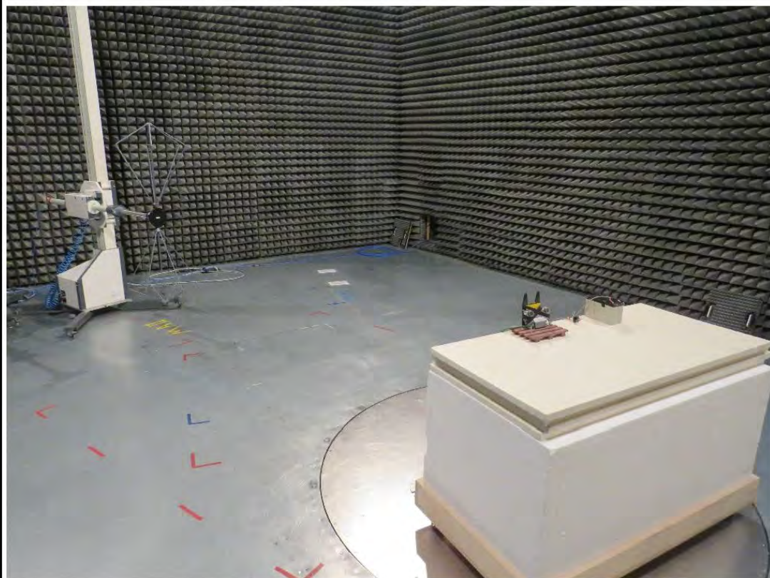
TEST SETUP Radiated emissions 30-200MHz
