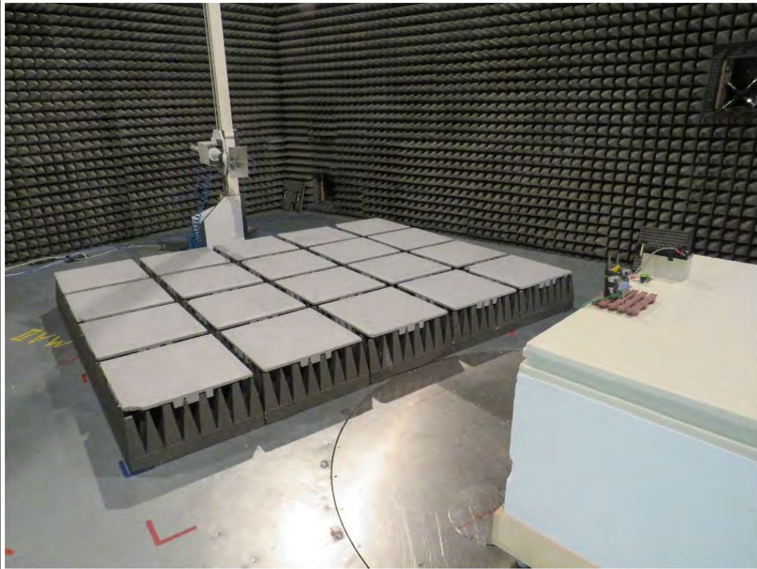
TEST SETUP Radiated emissions 1-10GHz
