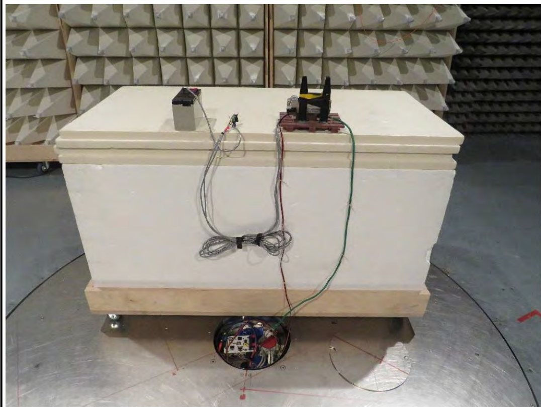
TEST SETUP Radiated emissions 1-10GHz - Turntable setup
