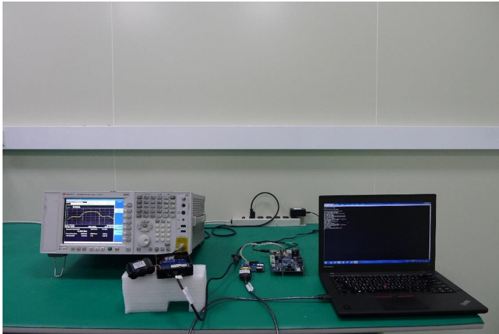
Description: Conducted Emission Test Setup
