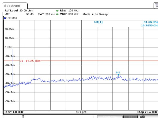
GFSK on channel 39
