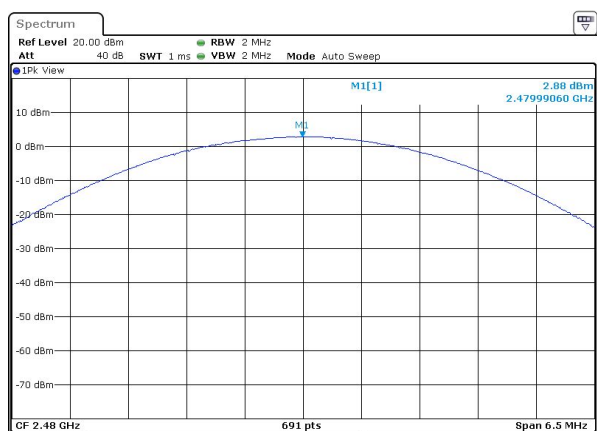
Peak output Power plot on channel 78 (3Mbps)
