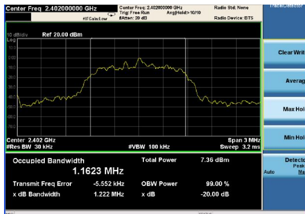
20dB Bandwidth plot on channel 00 (2Mbps)
