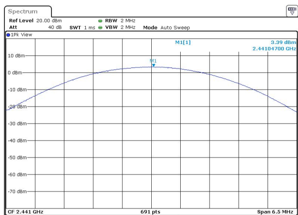
Peak output Power plot on channel 39 (3Mbps)
