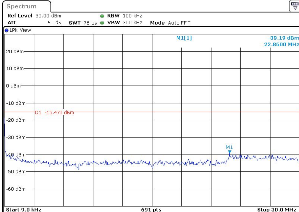
GFSK on channel 78
