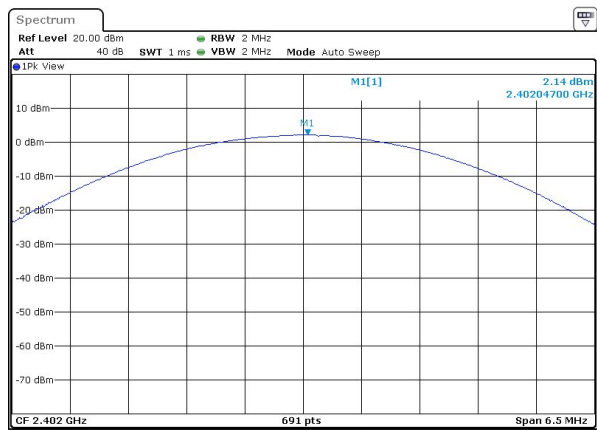
Peak output Power plot on channel 00 (3Mbps)
