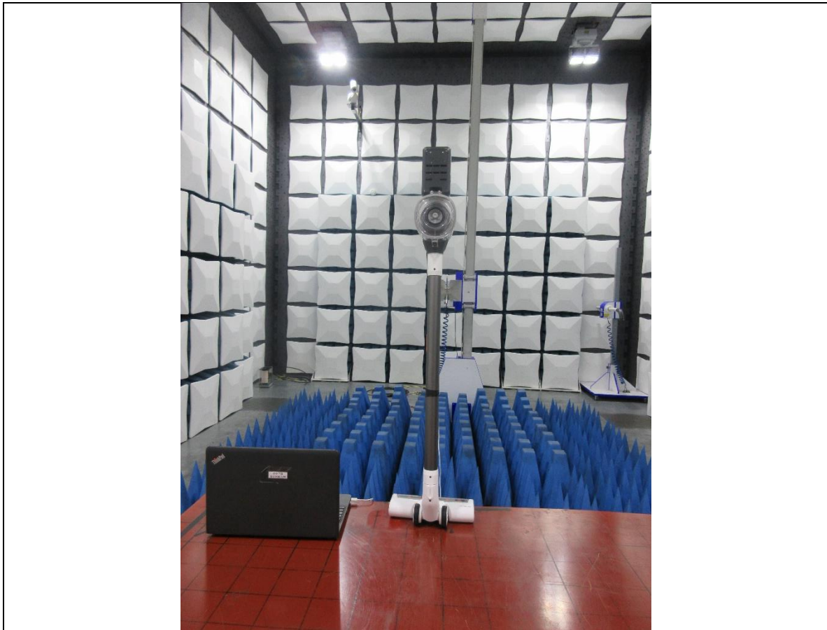
RADIATED RF MEASUREMENT SETUP (ABOVE 1 GHz- Z axis)
