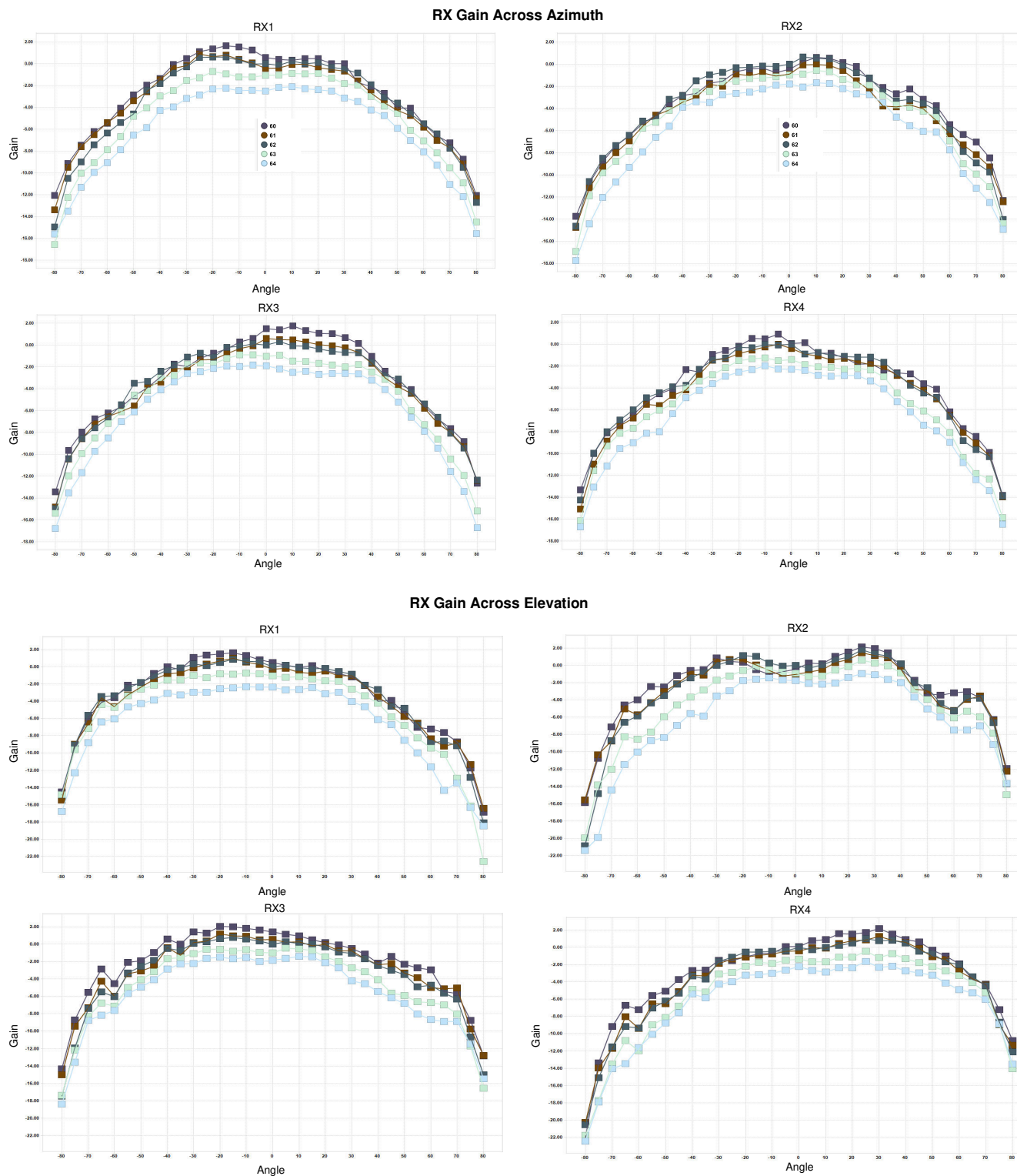
Figure 8-1. Receiver Antenna Radiation Pattern
