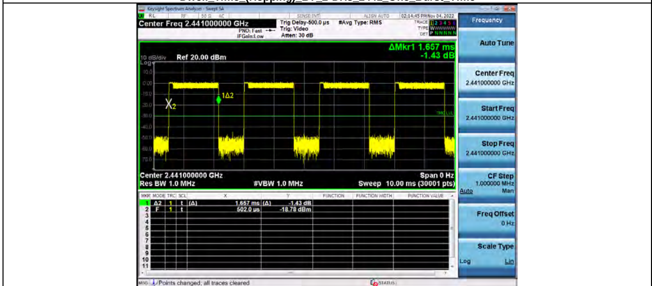
Dwell Time (Hopping) BT 2-DH3 2441 One Burst Time
