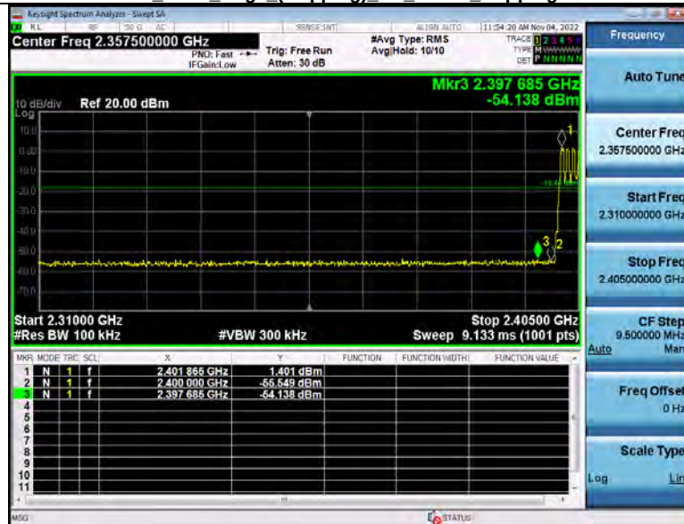
2 Band Edge (Hopping) BT 1-DH5 Hopping
