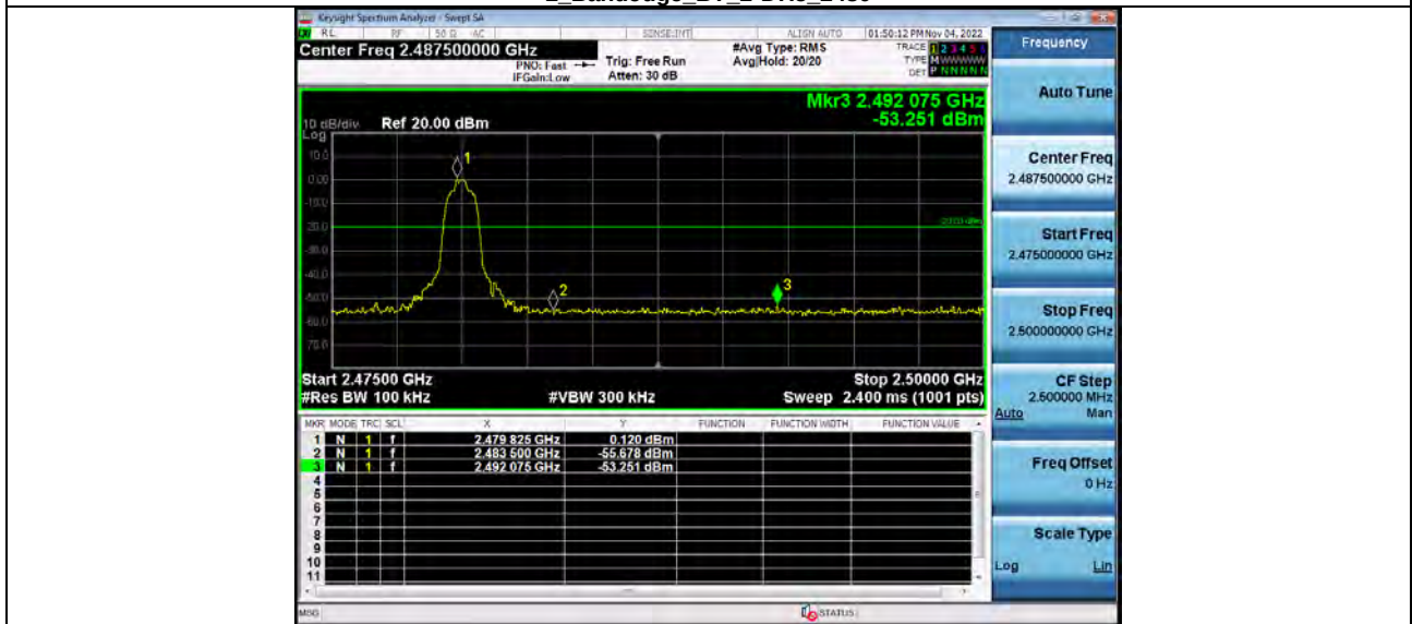
2 Bandedge BT 2-DH5 2480
