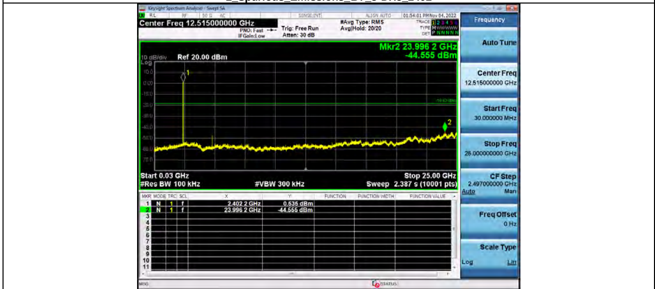
2 Spurious Emissions BT 3-DH5 2402
