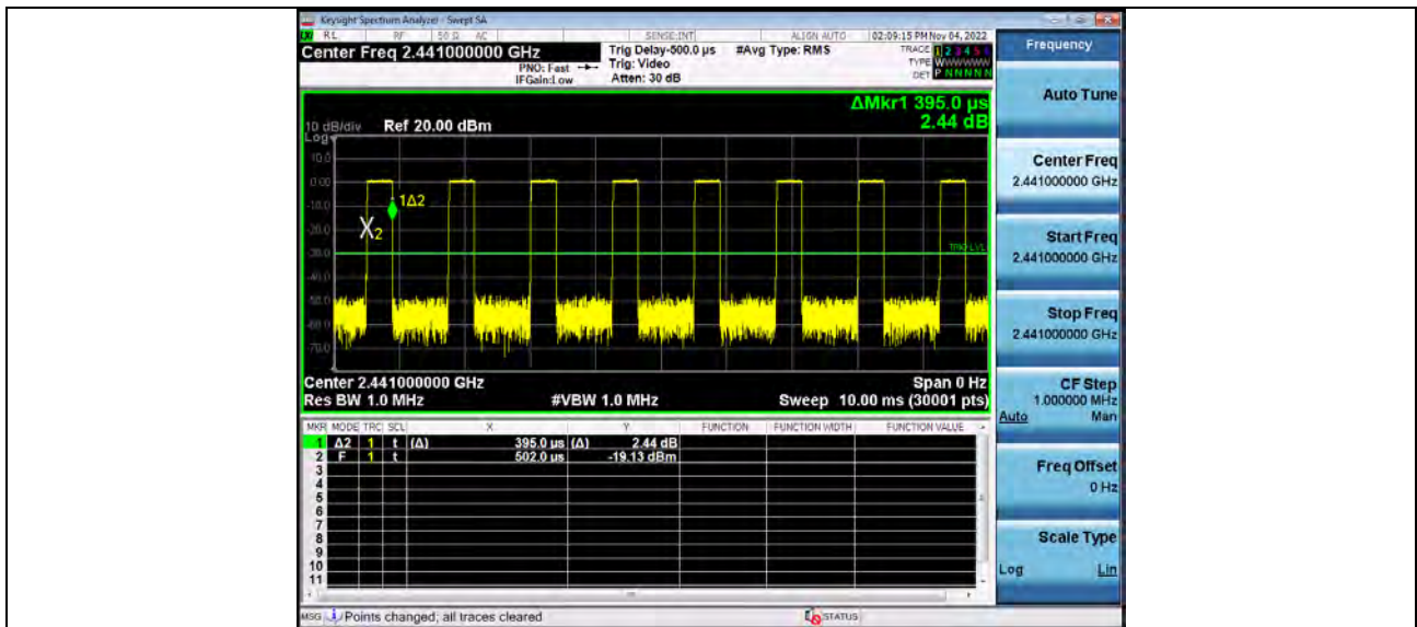
Dwell Time (Hopping) BT 2-DH5 2441 One Burst Time
