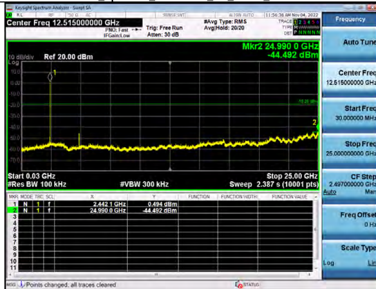
2 Spurious Emissions BT 1-DH5 2441
