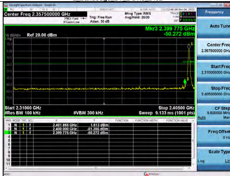
2 Bandedge BT 1-DH5 2402
