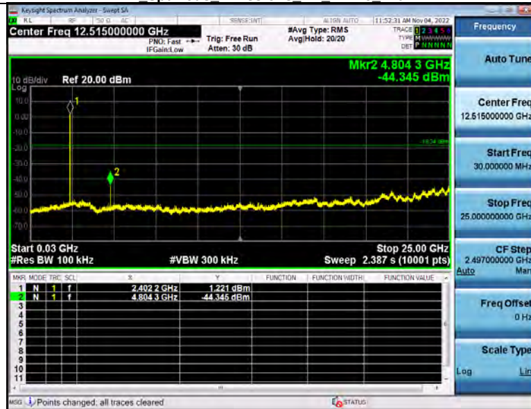
2 Spurious Emissions BT 1-DH5 2402
