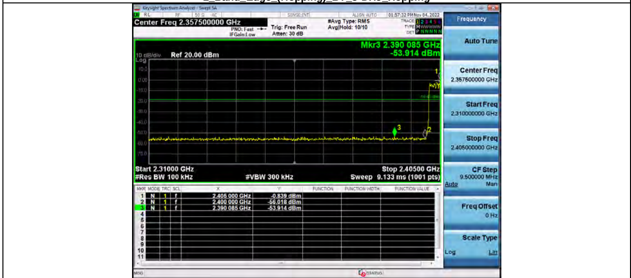
2 Band Edge (Hopping) BT 3-DH5 Hopping
