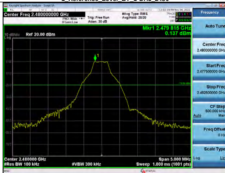
2 Bandedge BT 1-DH5 2480
