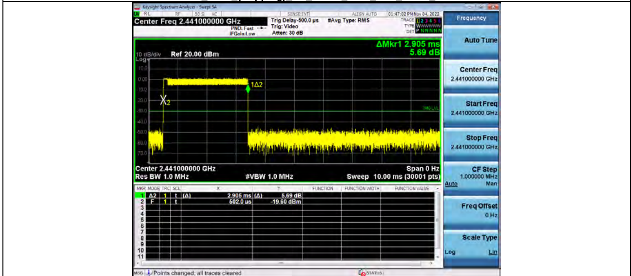
Dwell Time (Hopping) BT 2-DH5 2441 One Burst Time
