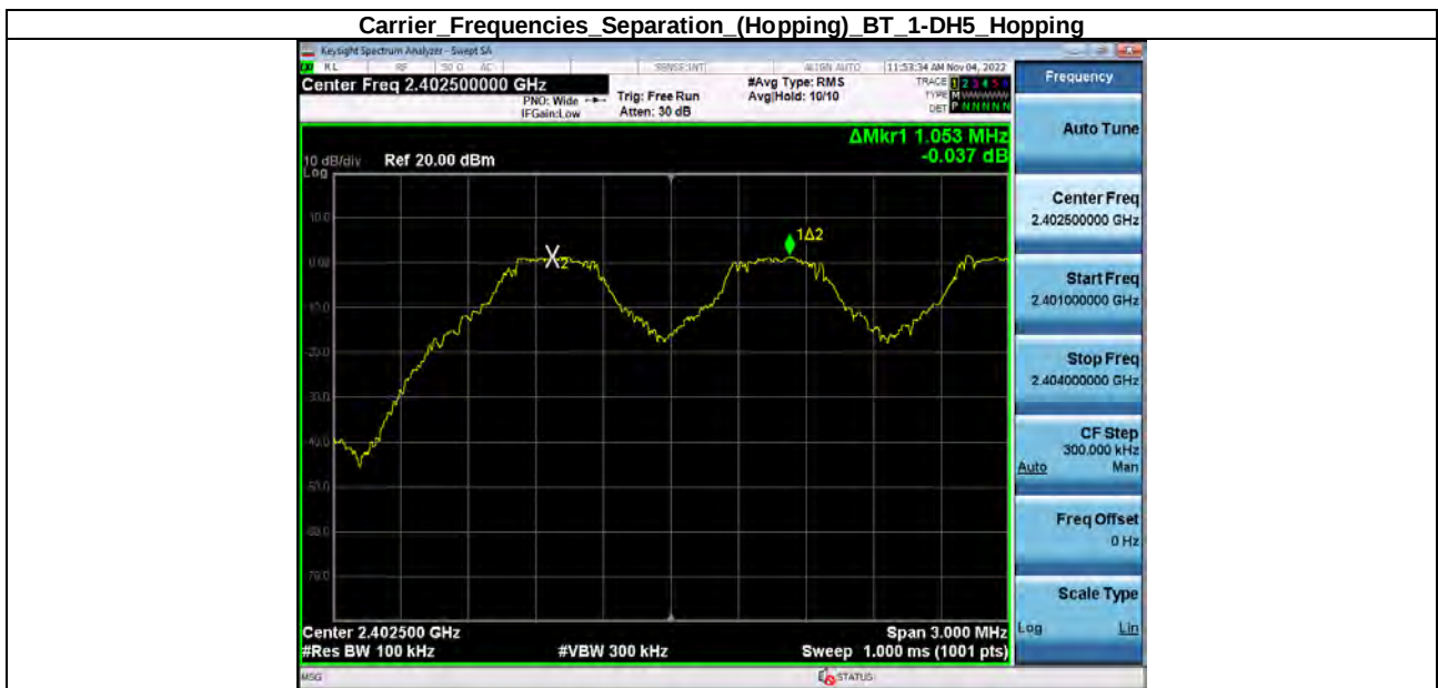
Carrier Frequencies Separation (Hopping) BT 1-DH5 Hopping
