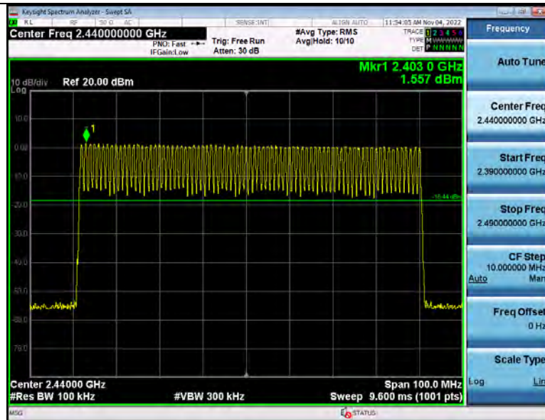
2 Band Edge (Hopping) BT 1-DH5 Hopping
