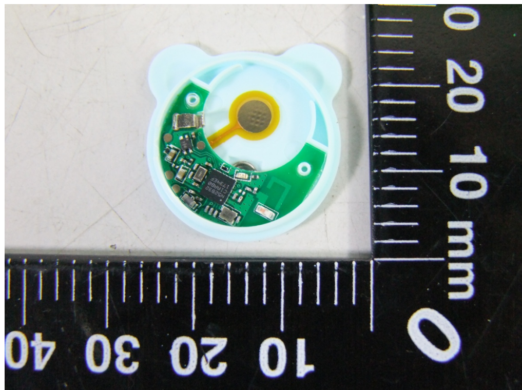
Photo 2 Inside of EUT (RIT-P02-MED)
