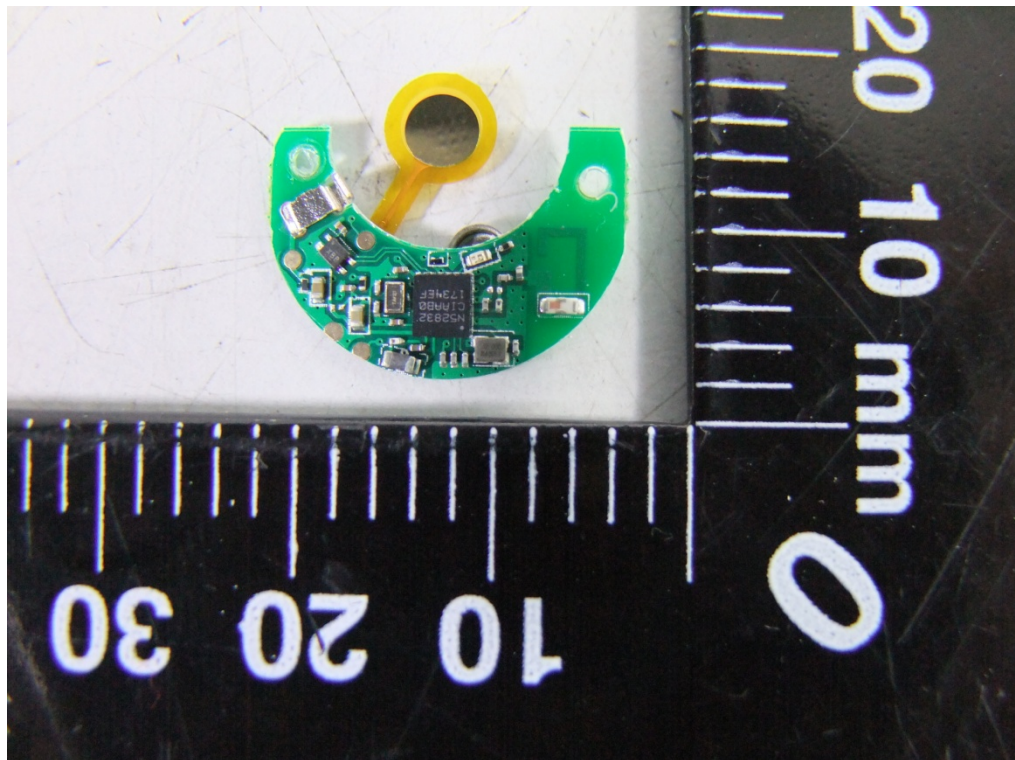
Photo 3 Inside of EUT (RIT-P02-MED)
