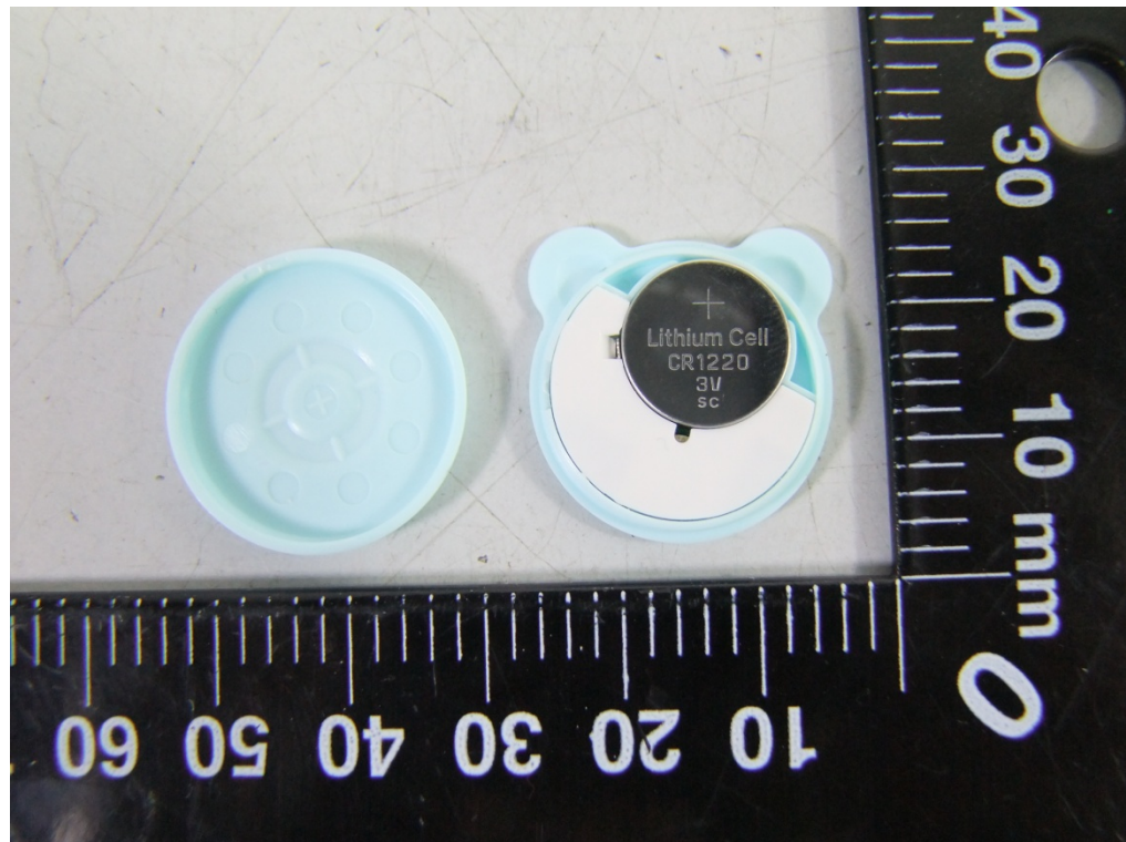
Photo 1 Inside of EUT (RIT-P02-MED)
