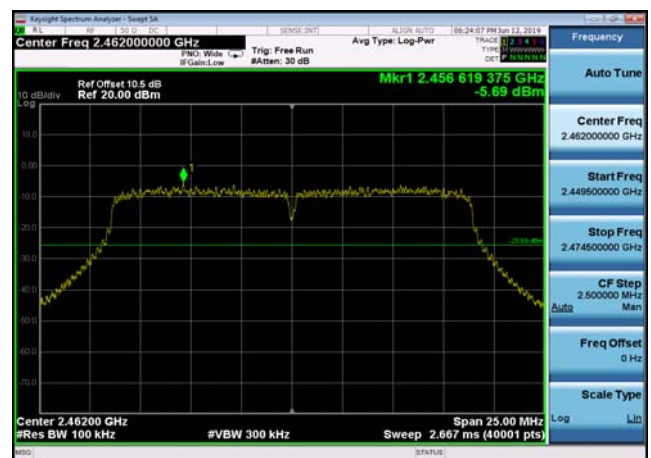
,Plot 1,Reference Level-802.11n(HT20) ,2462MHz,Ant1
