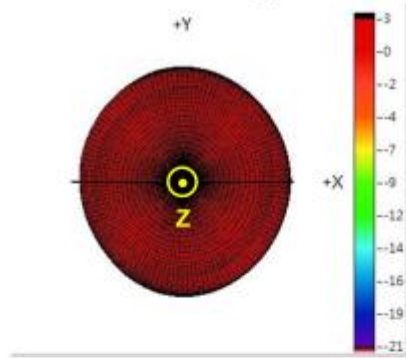
7-1. 3D Gain Pattern @ 2442 MHz (unit: dBi)
