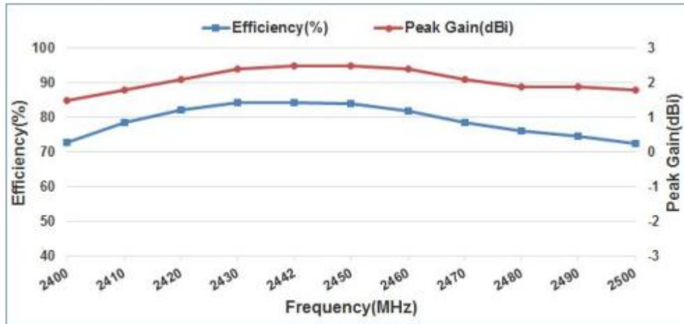
7-3. 3D Efficiency vs. Frequency
