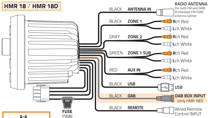
12 PIN HARNESS
