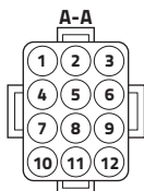
12 Pin Harness
