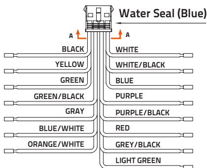
15 PIN HARNESS
