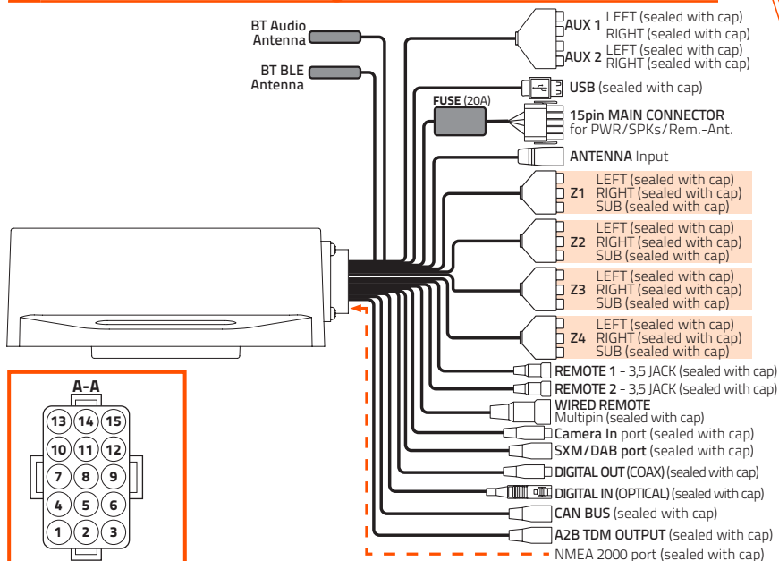
15 pin Harness pin out
