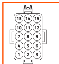
15 pin Harness pin out
