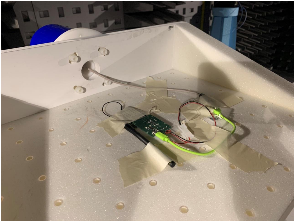
EUT test set up position during radiated emission above 1 GHz
