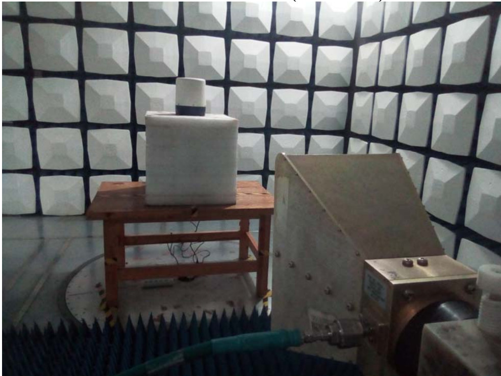
RE Above 1GHz Front View(1GHz-40GHz)
