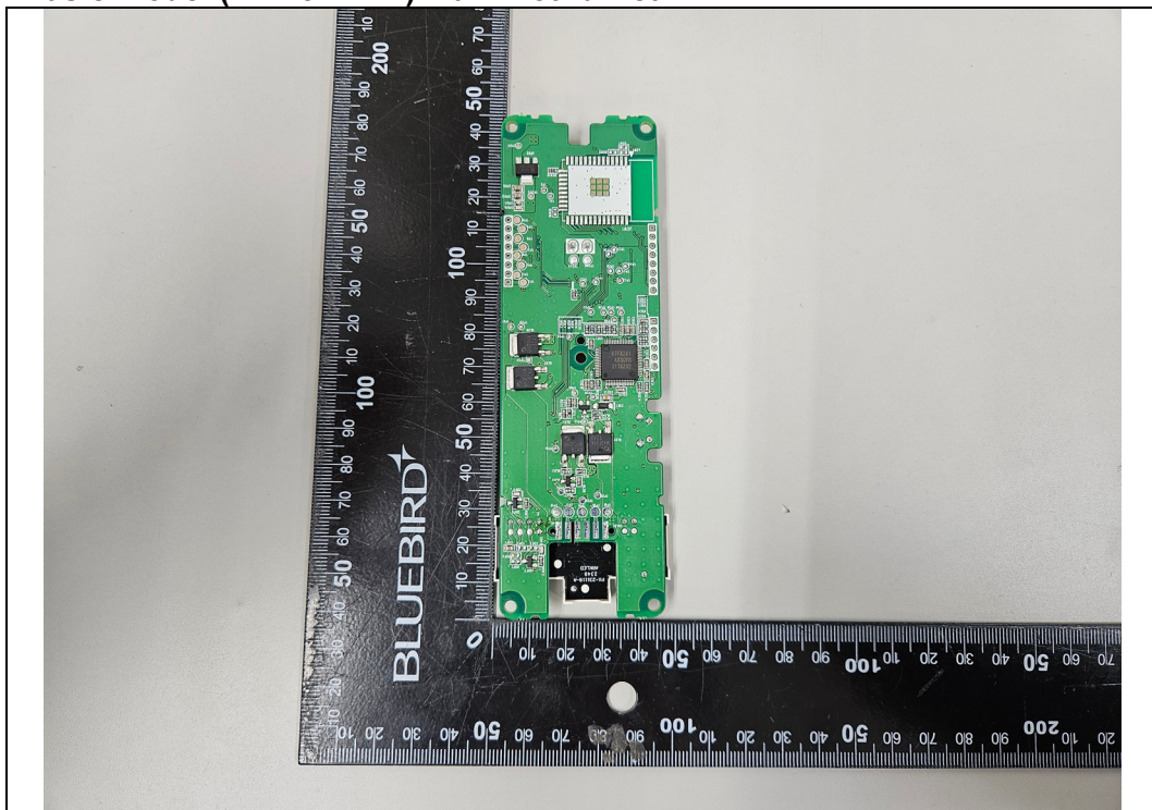
Basic model (EME511-KP) Main Board Rear
