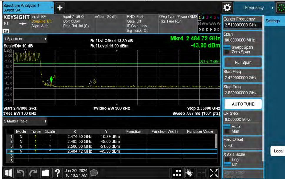
2DH5-Ant1-Hop 2480-PASS
