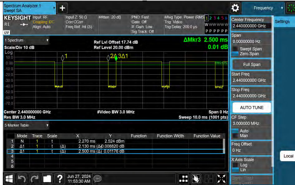
NTNV-BLE 2M-Ant1-2440
