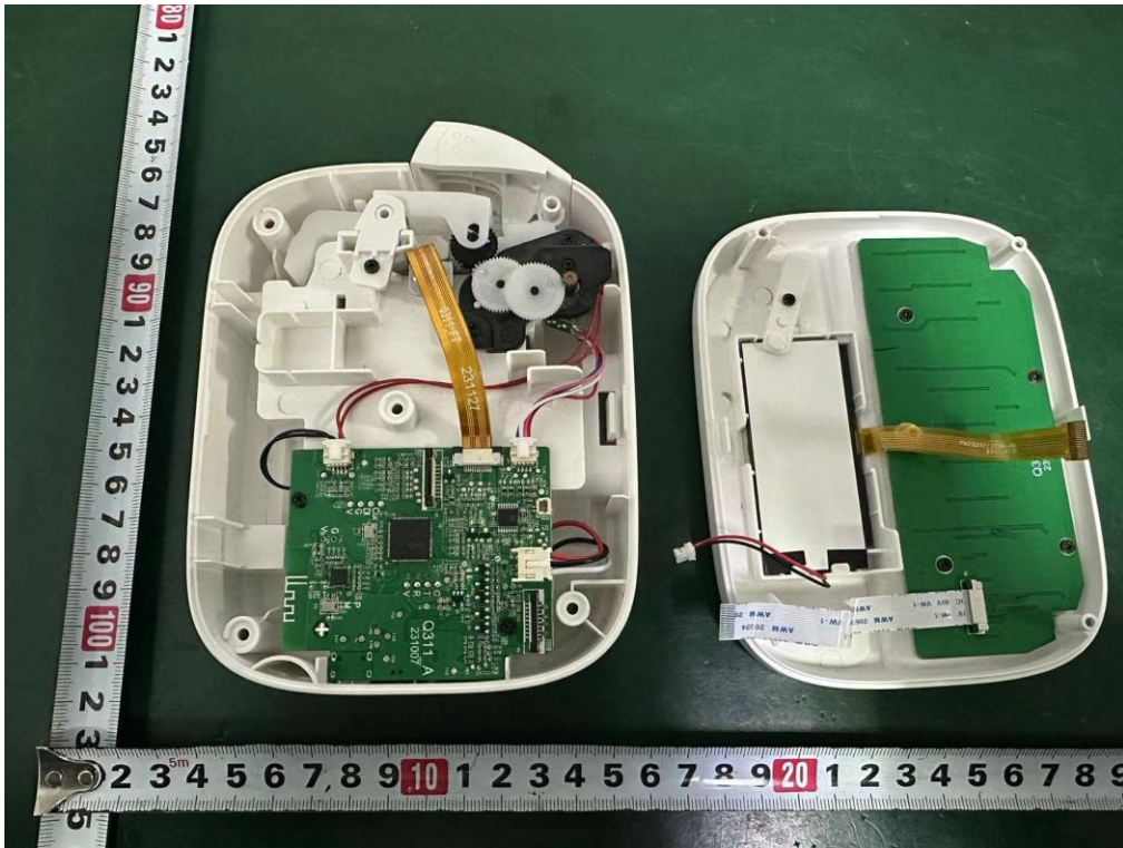
Internal photos M/N: M950
