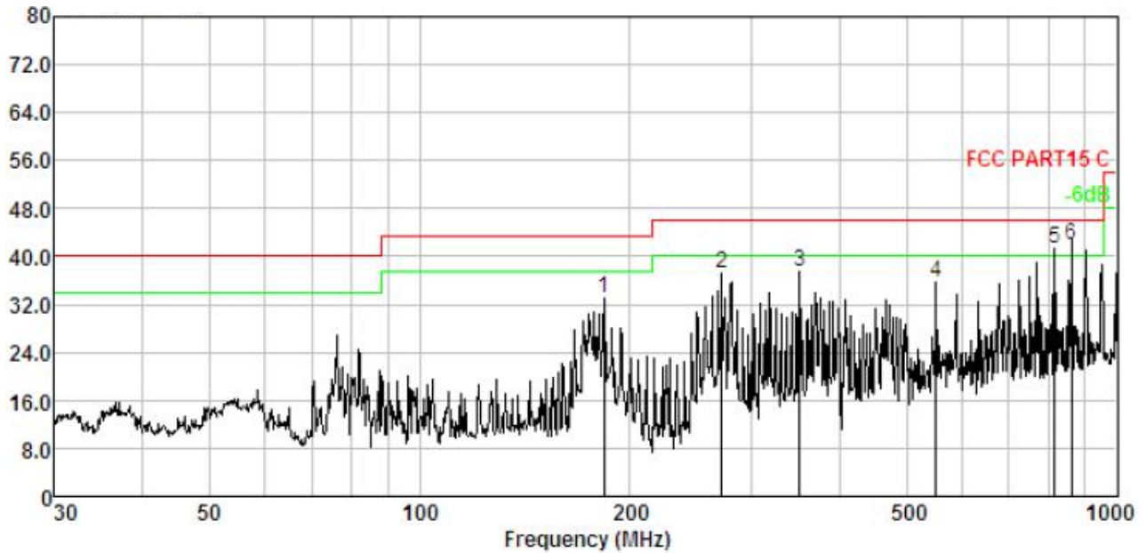
Test plot for Horizontal: GFSK(2402MHz)
