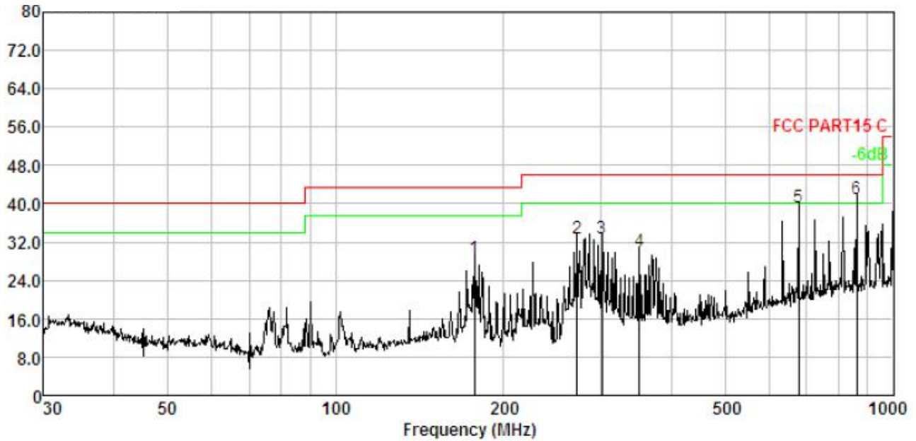
Test plot for Vertical: GFSK(2402MHz)
