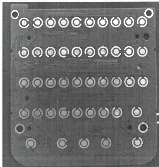
New PCB:
