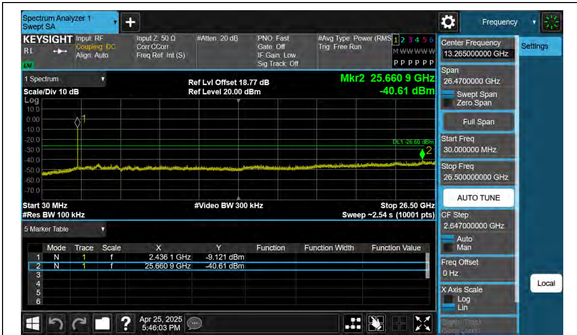
11N40SISO-Ant1-2452-30~26500-PASS
