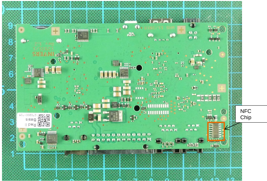
181948_eut17.JPG : EUT main unit PCB A top view
