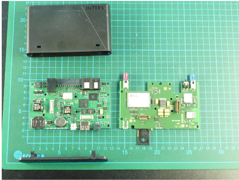
181948_eut12.JPG : EUT main unit inside view 3
