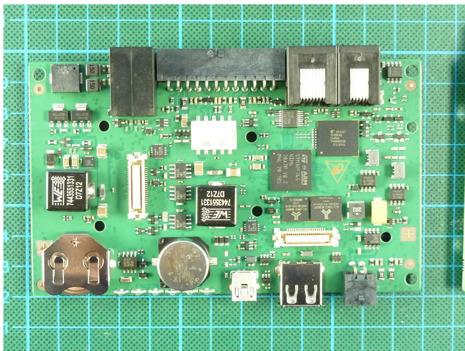
181948_eut15.JPG : EUT main unit PCB A bottom view
