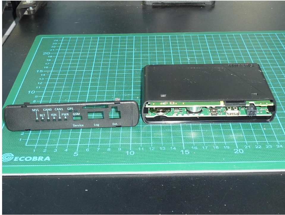
181948_eut10.JPG : EUT main unit inside view 1
