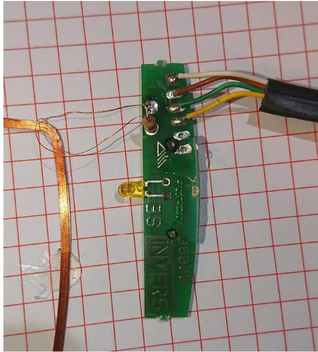
181948_eut24.jpg : EUT NFC antenna PCB view 1 (Photo delivered by the applicant)
