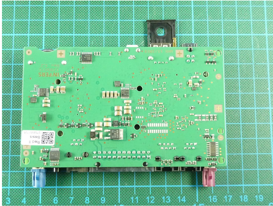
181948_eut14.JPG : EUT main unit PCB's view 2
