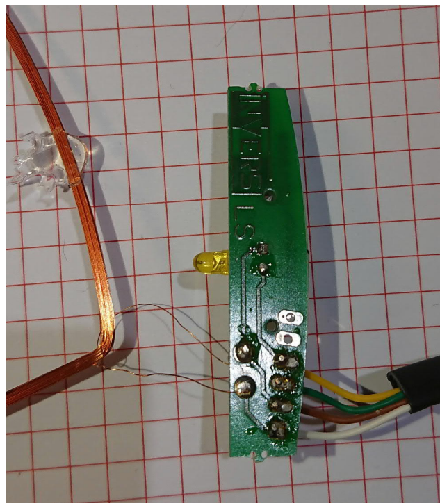
181948_eut25.jpg : EUT NFC antenna PCB view 2 (Photo delivered by the applicant)
