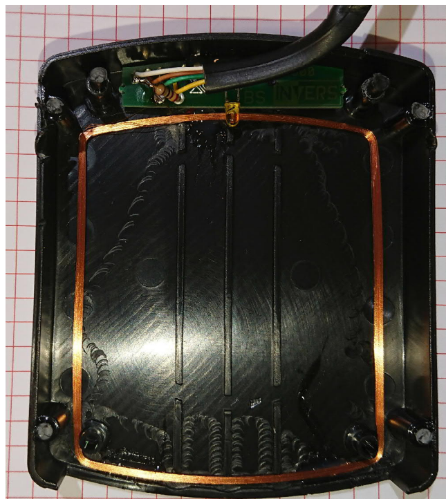
181948_eut23.jpg : EUT NFC antenna inside view 2 (Photo delivered by the applicant)
