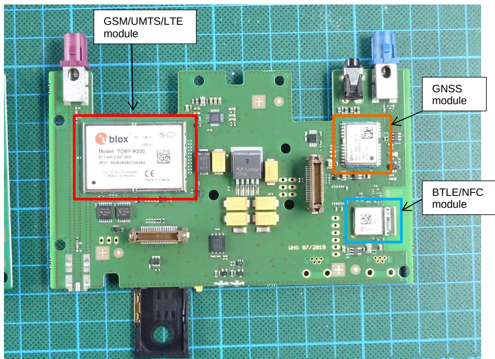
181948_eut16.JPG : EUT main unit PCB B bottom view
