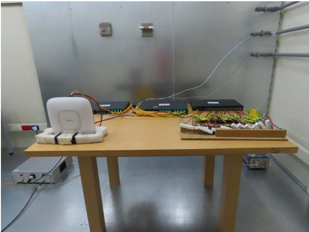
Set Up Photo of Conducted Emission BU Chassis
