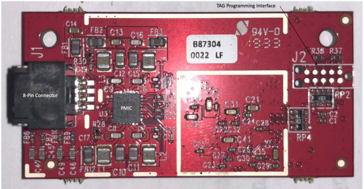
Figure 2. Key Module Component Placement (Back)
