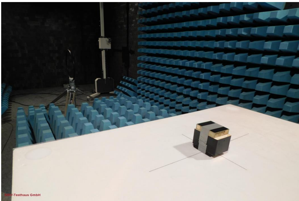
Picture 4: CDC, radiated emission test 9 kHz -30 MHz (front view)
