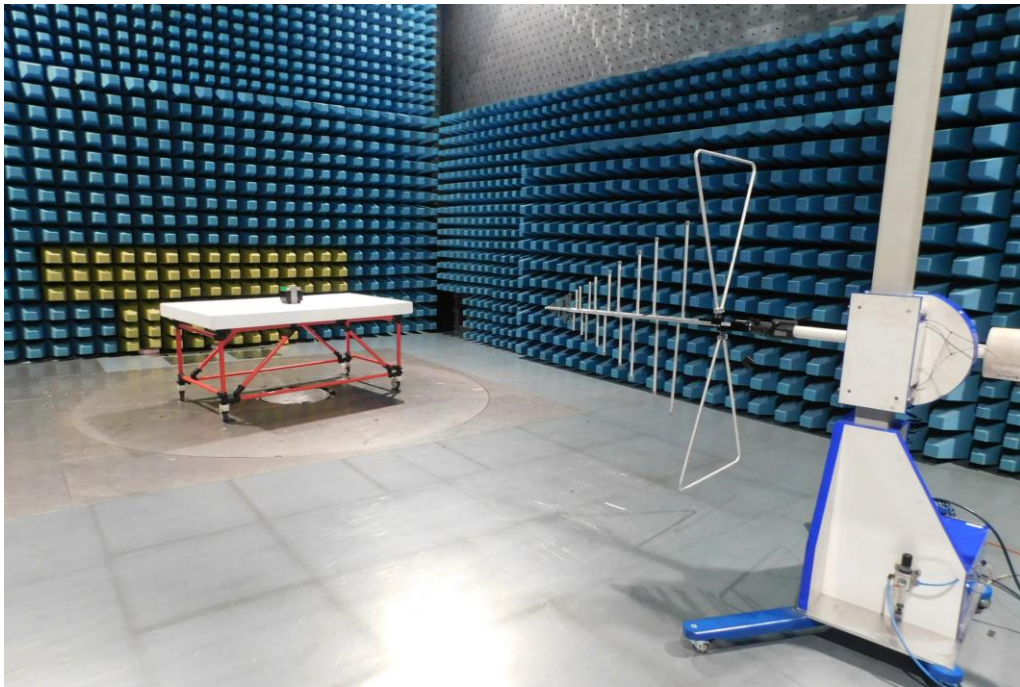
Picture 7: SAC, radiated emission test 30 MHz – 1 GHz (rear view)
