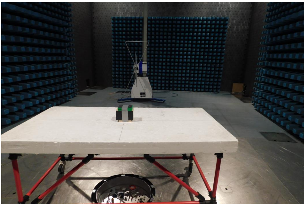
Picture 6: SAC, radiated emission test 30 MHz – 1 GHz (front view)
