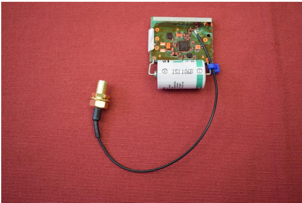
Picture 12: Module with antenna cable – top view
