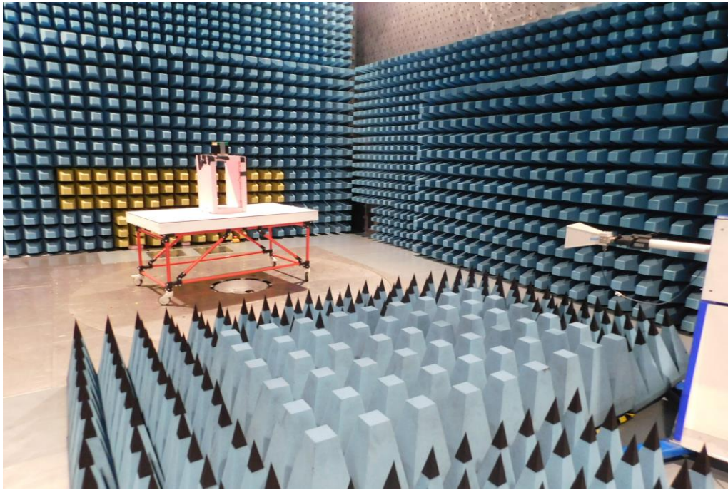
Picture 9: SAC, radiated emission test 1 GHz – 12.5 GHz (rear view)
