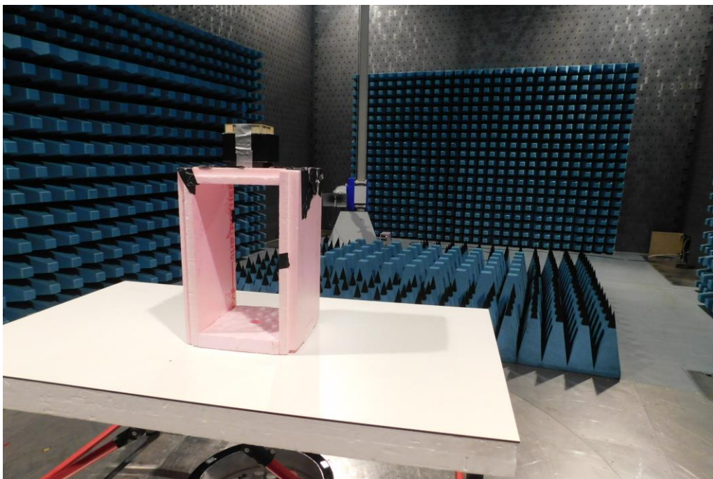
Picture 8: SAC, radiated emission test 1 GHz – 12.5 GHz (front view)
