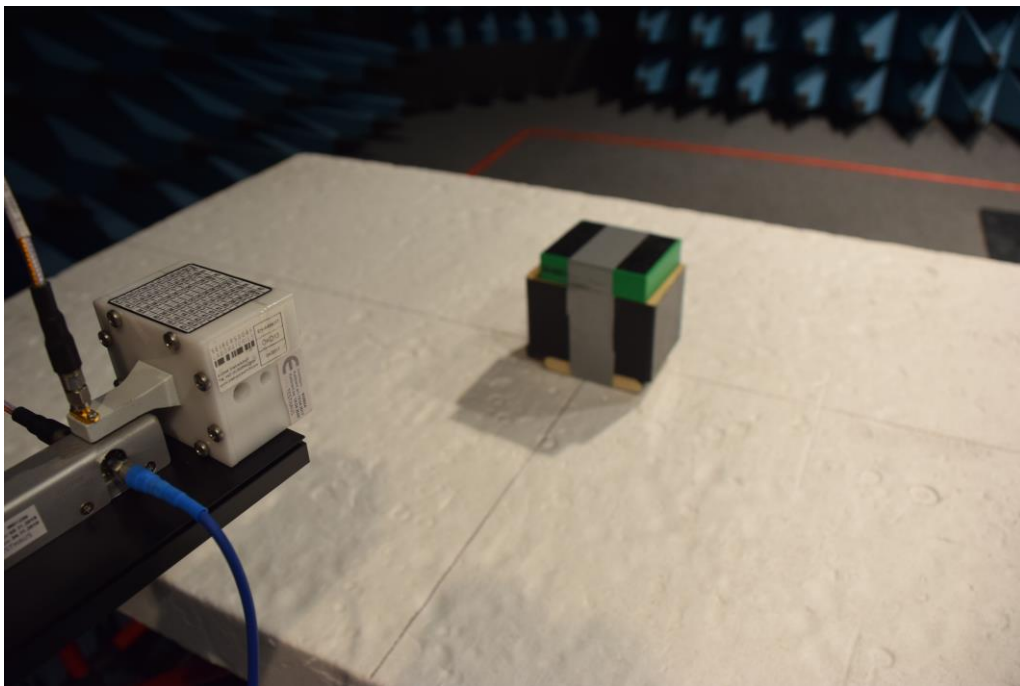
Picture 10: AC, exploratory measurement 12.5 GHz – 25 GHz (top view)
