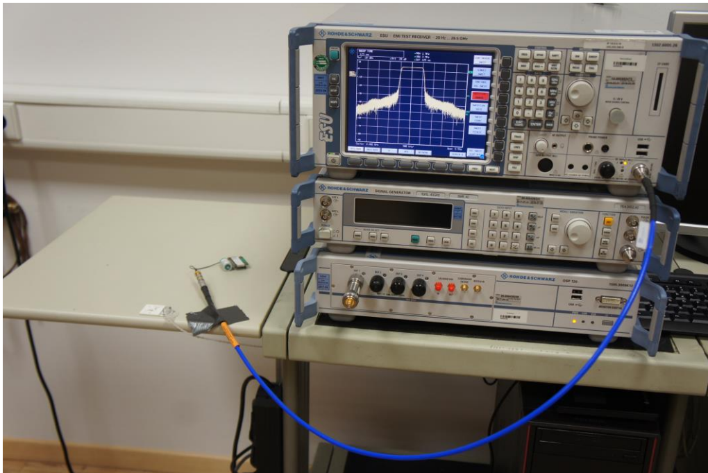
Picture 11: Conducted measurements (front view)
