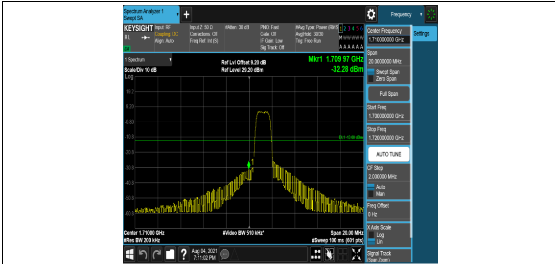
Band4-10MHz-16QAM-20000-6-0-Low--32.28-PASS
