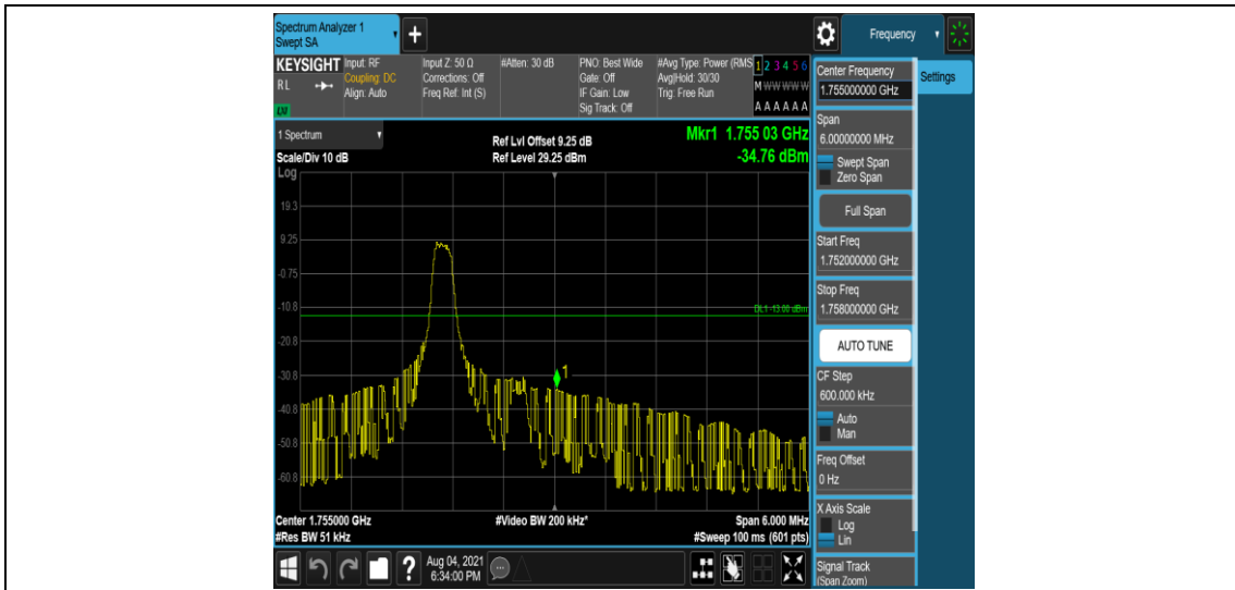
Band4-3MHz-16QAM-20385-1-0-High--34.76-PASS
