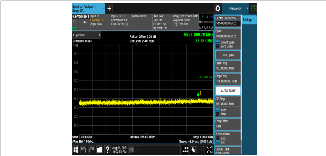
Band4-1.4MHz-QPSK-20175-1-0-Low-30-1000--33.78-PASS
