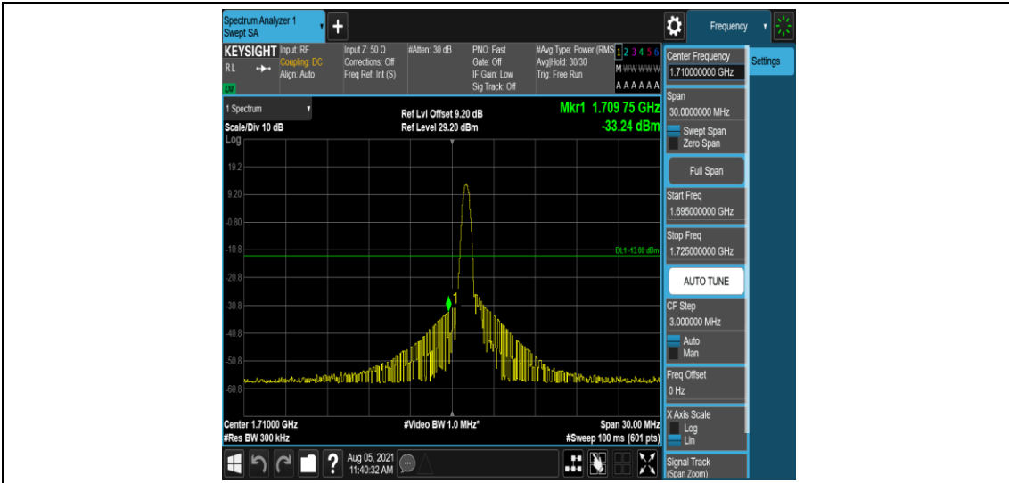
Band4-15MHz-QPSK-20025-1-0-Low--33.24-PASS
