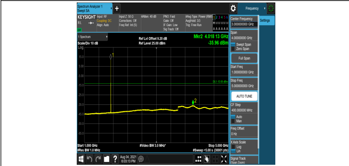
Band4-1.4MHz-QPSK-20175-1-0-Low-1000-5000--35.96-PASS
