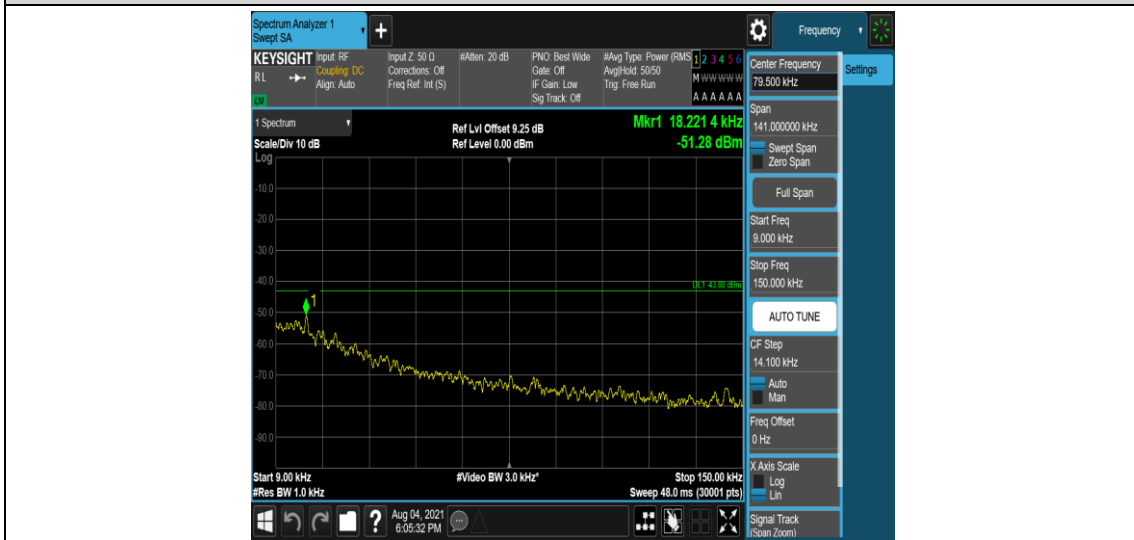
Band4-1.4MHz-QPSK-20393-1-0-High-0.009-0.15--51.28-PASS
