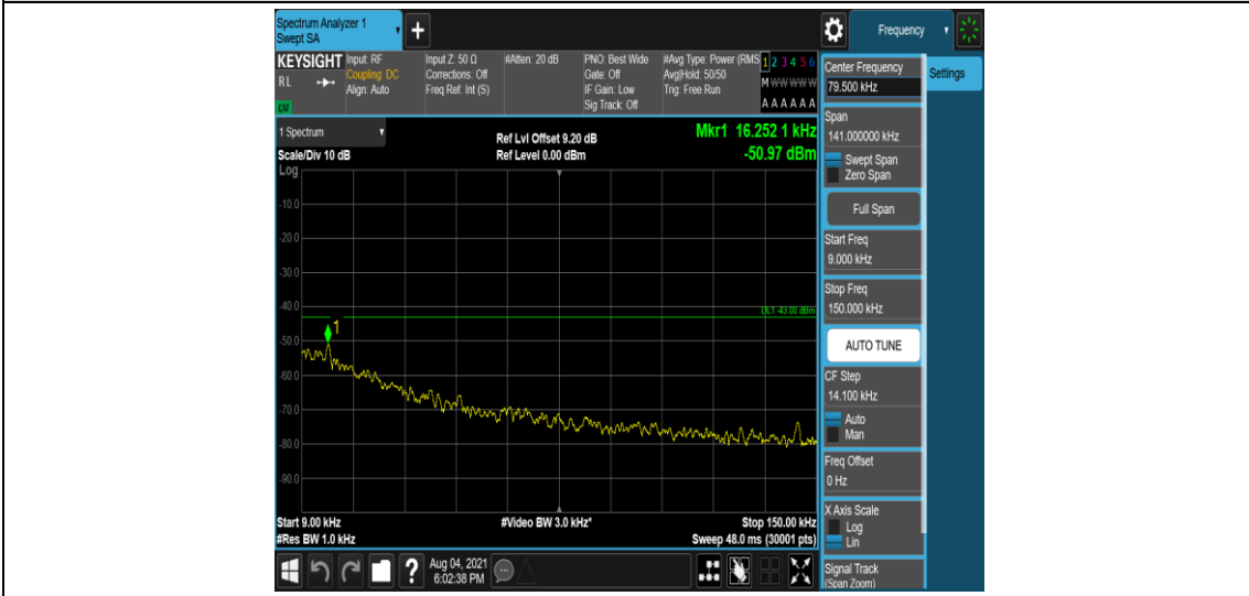
Band4-1.4MHz-QPSK-20175-1-0-Low-0.009-0.15--50.97-PASS
