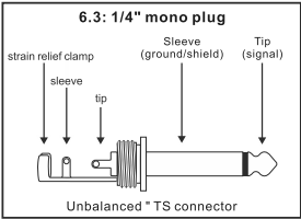
6.3: 1/4 inch mono plug
