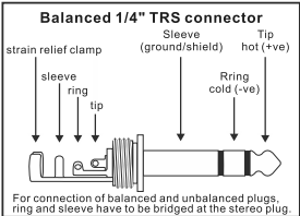
Balanced 1/4 inch TRS connector
