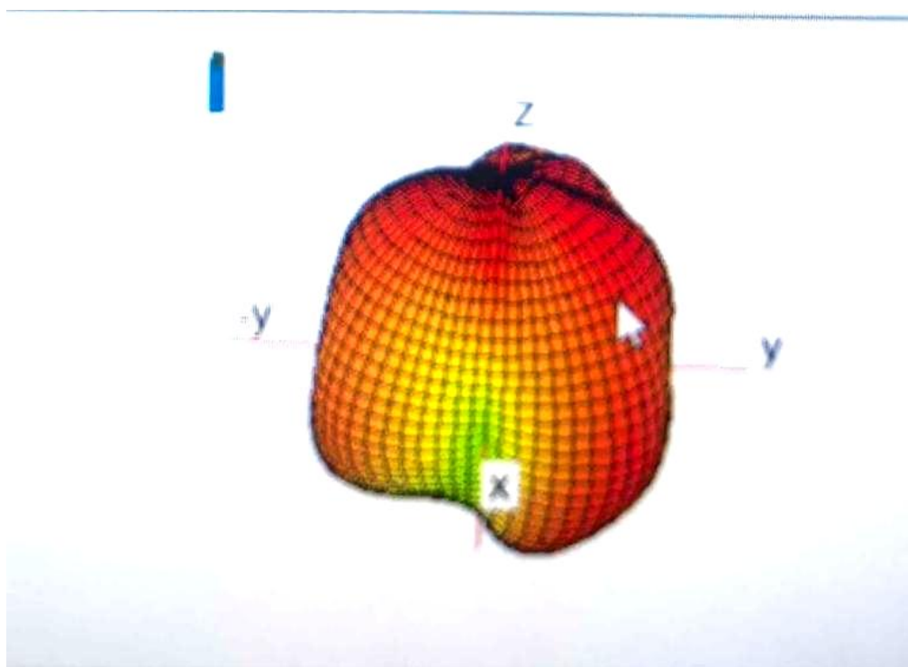
Radiation Pattern(5G)
