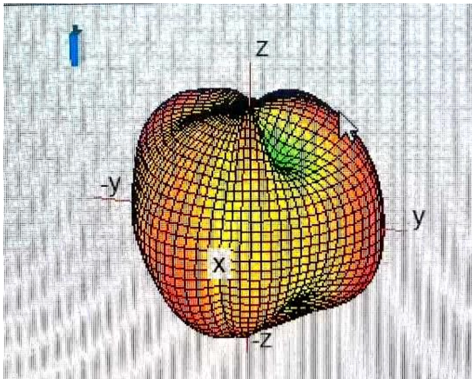
Radiation Pattern(5G)
