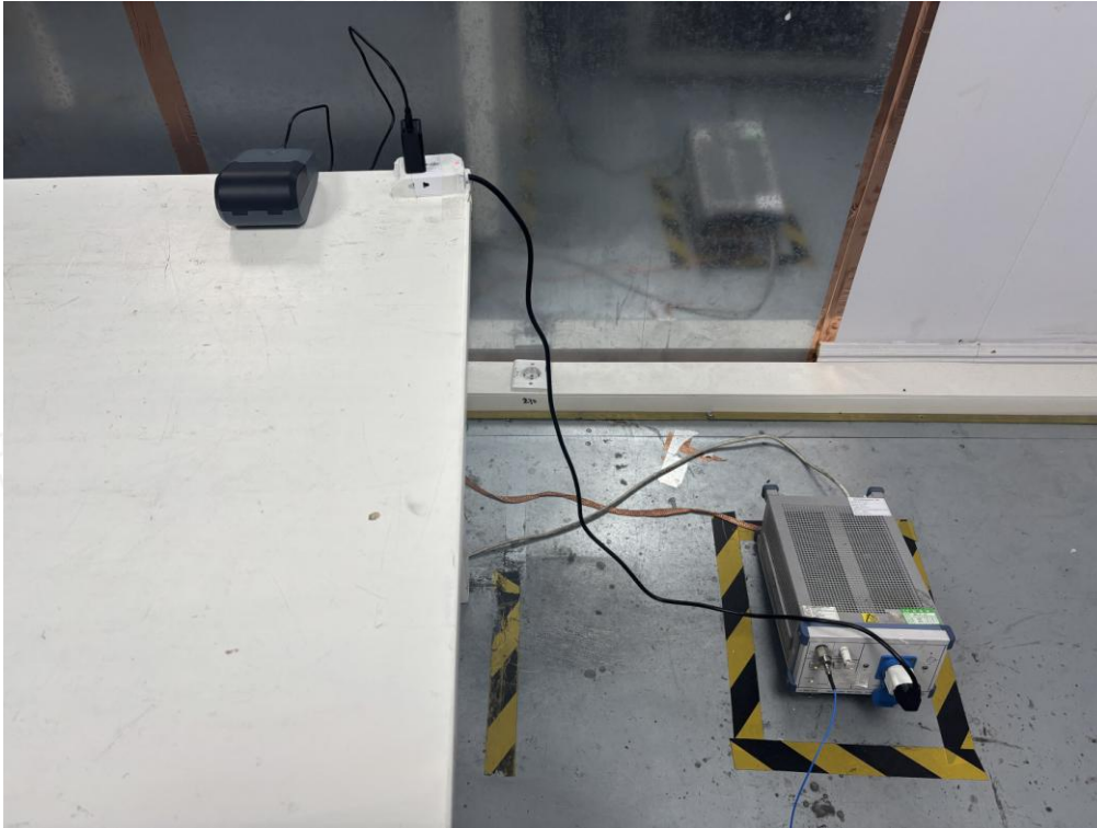
Fig. 3 Test Setup Photo(s) of RF
