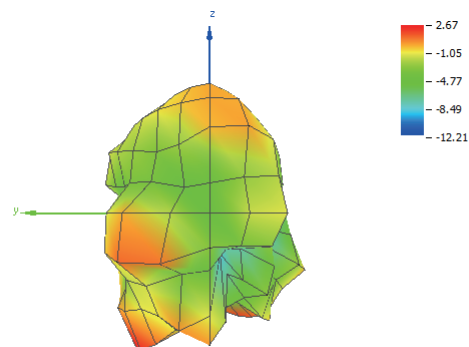
(2.40 GHz): Theta = 90, Phi = 180
