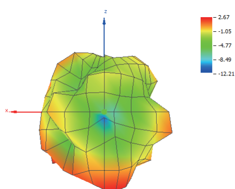
(2.40 GHz): Theta = 90, Phi = 90
