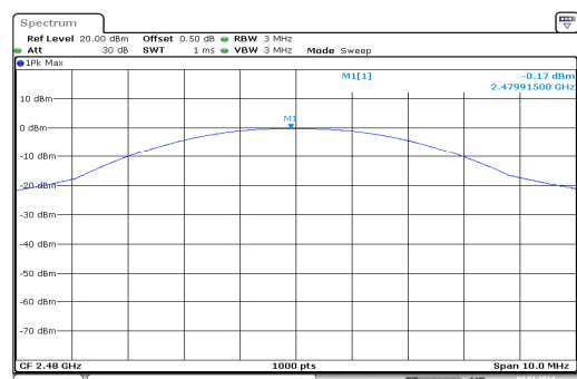
GFSK_High_DH1
