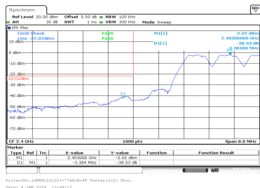
GFSK_Hopping_Lower_DH1
