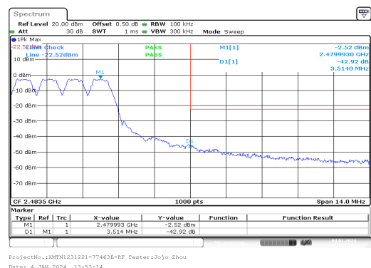
GFSK_Hopping_Upper_DH1
