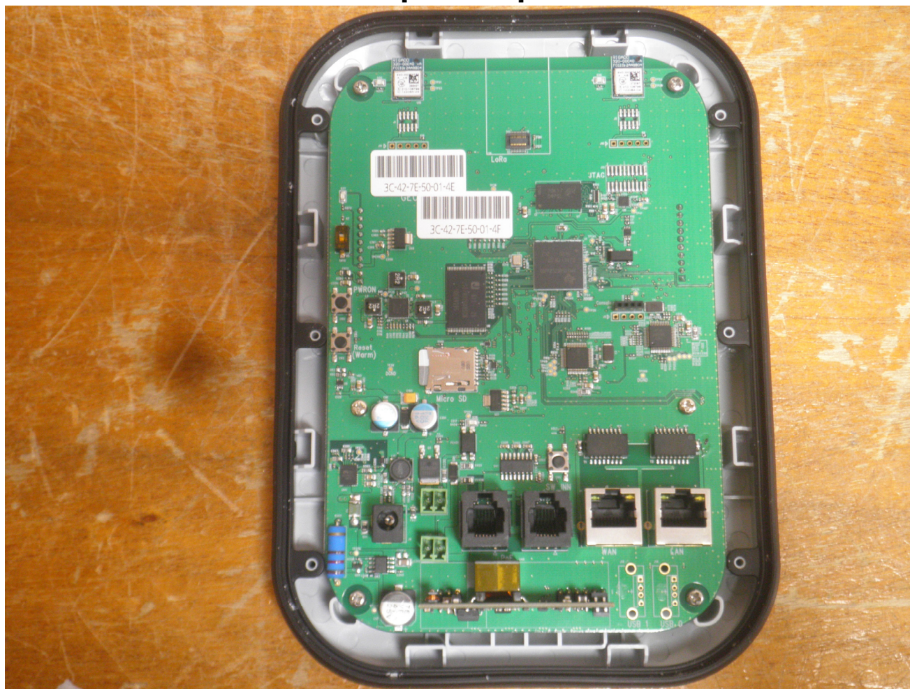
[ Inside View ]
