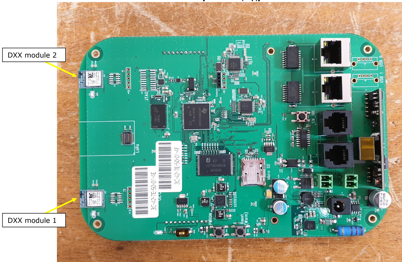
[Main board(Top)]
