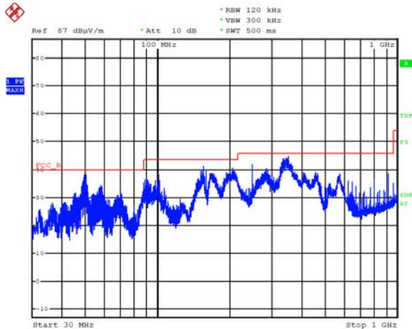
Horizontal
