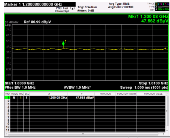
Vertical(960-1 610 MHz)
