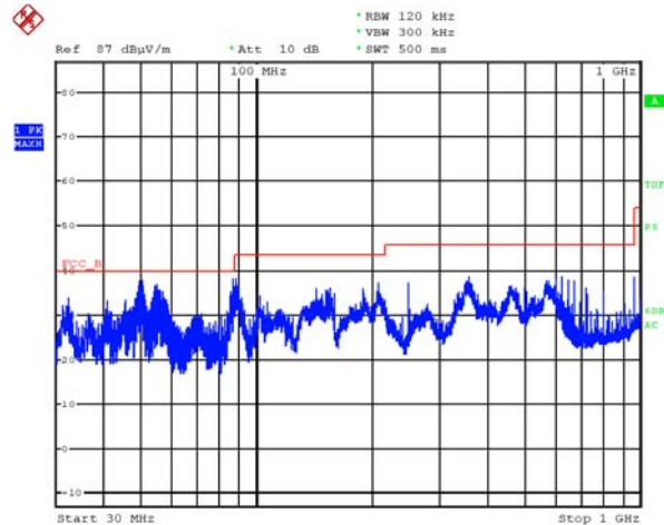
Vertical
