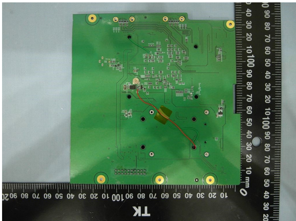
(34) EUT Photo
