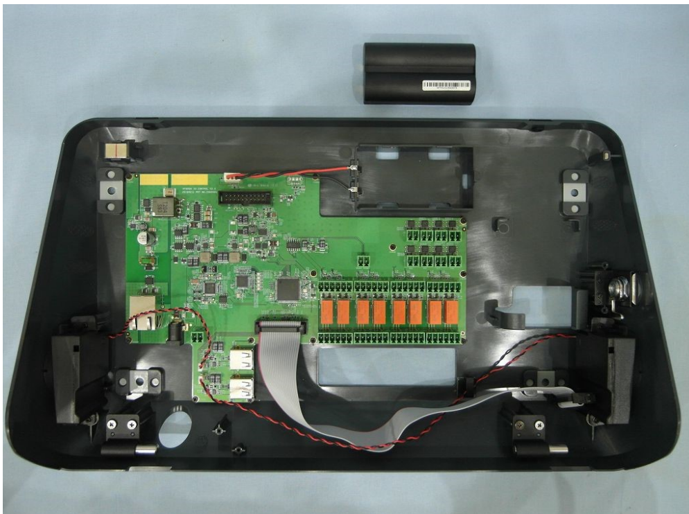
(42) EUT Photo
