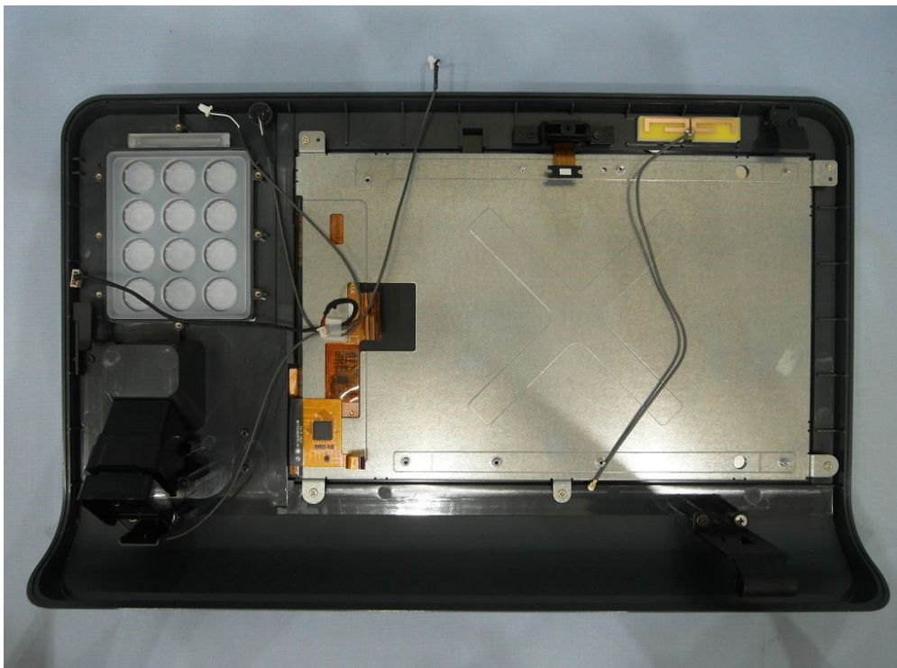
(32) EUT Photo
