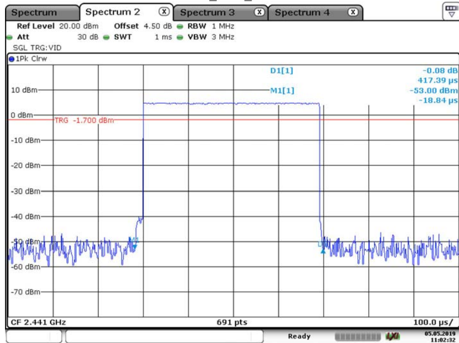
GFSK_DH1_Middle
