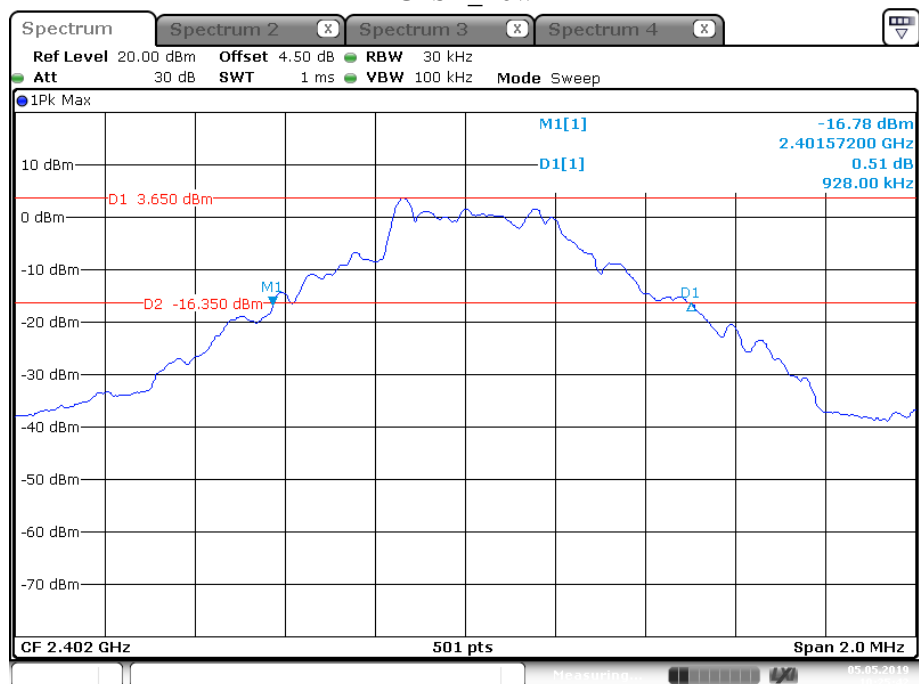
GFSK_Low
