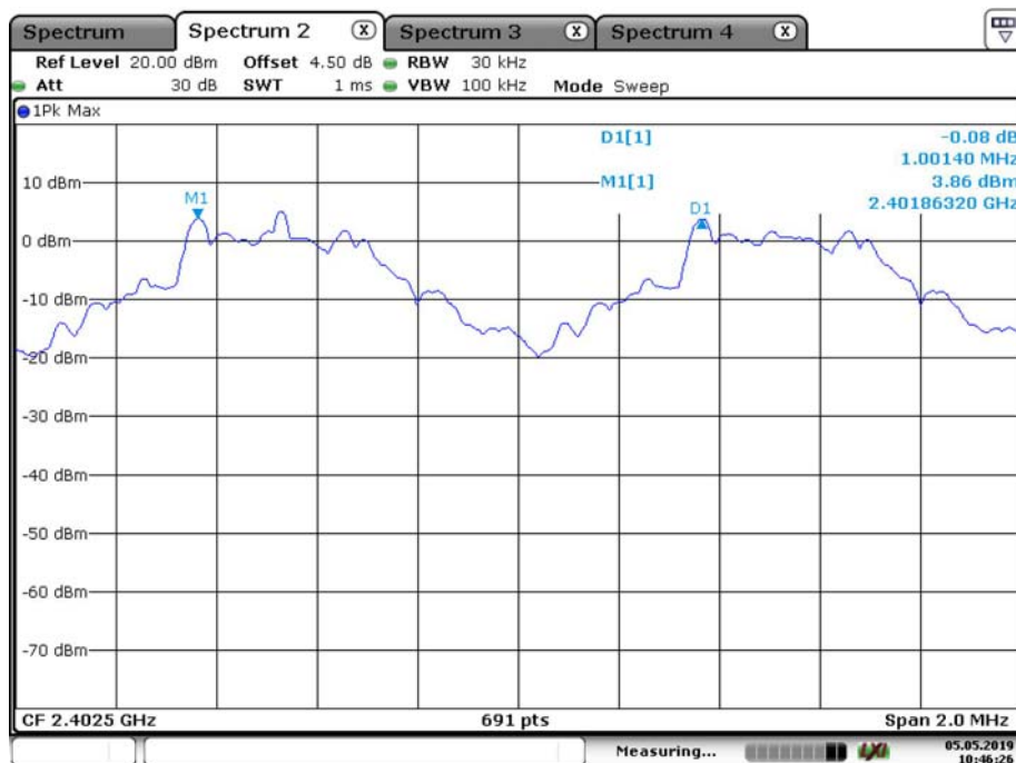
GFSK_Low
