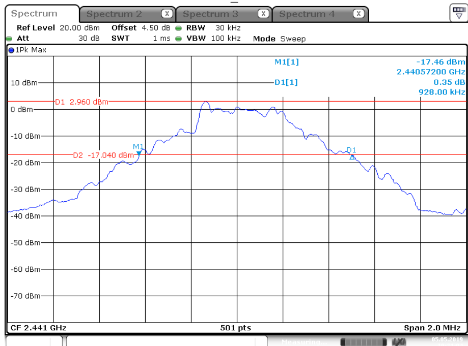
GFSK_Middle
