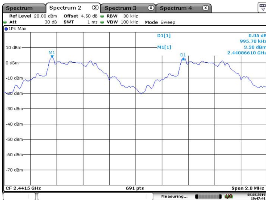
GFSK_Middle
