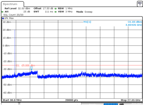
10MHz_Low_QPSK_1@0(30MHz~27.55GHz)
