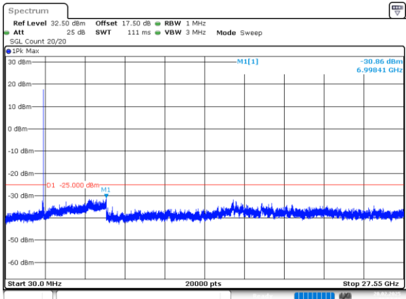
10MHz_High_QPSK_1@0(30MHz~27.55GHz)
