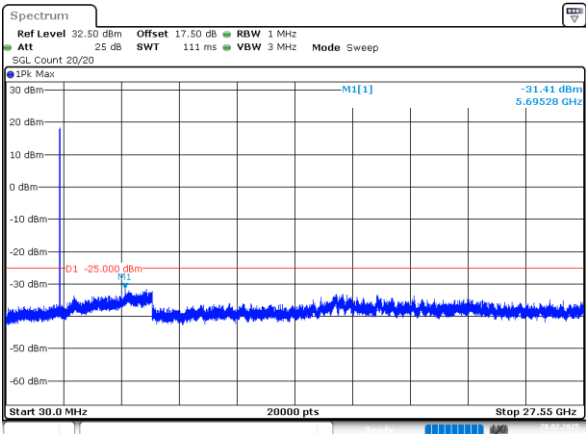
10MHz_Middle_QPSK_1@0(30MHz~27.55GHz)
