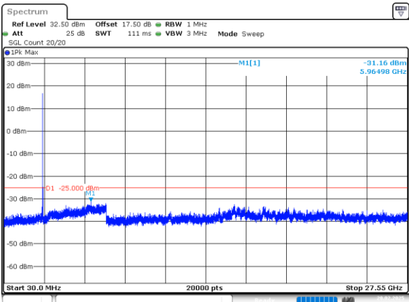
5MHz_High_QPSK_1@0(30MHz~27.55GHz)
