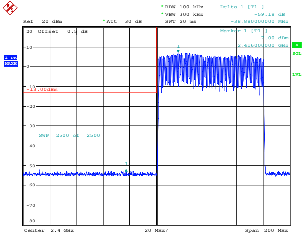
DH1_Hopping_Lower
