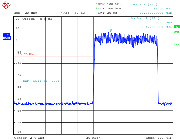
3DH1_Hopping_Lower
