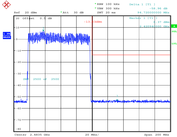
3DH1_Hopping_Upper
