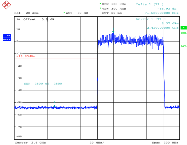
2DH1_Hopping_Lower
