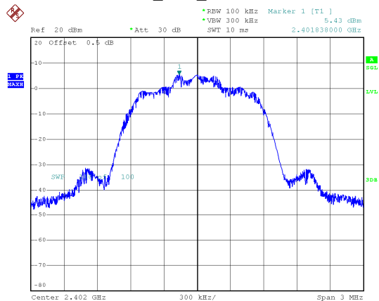
3DH1_Low_Reference Level
