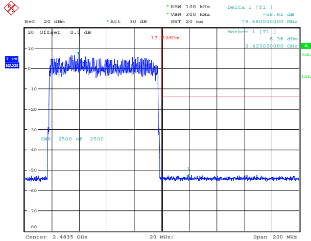
2DH1_Hopping_Upper
