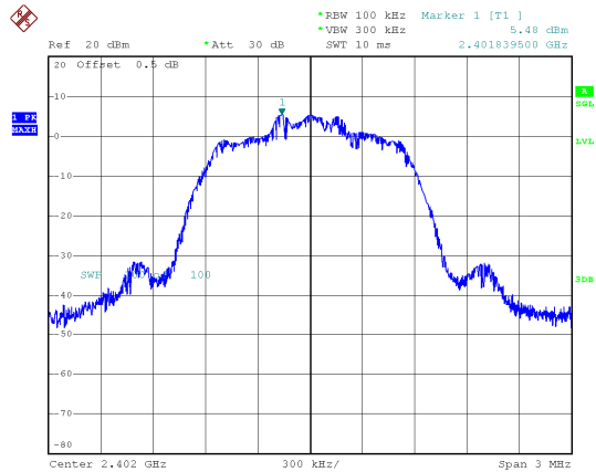
2DH1_Low_Reference Level
