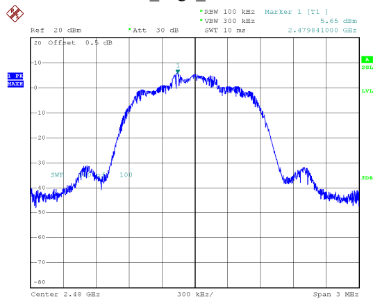
3DH1_High_Reference Level
