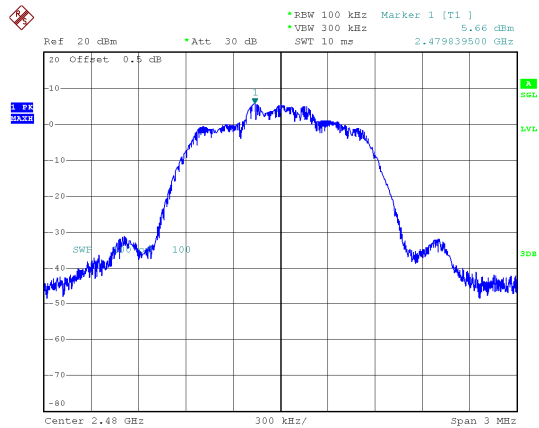
2DH1_High_Reference Level
