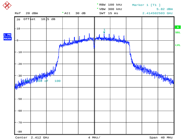
802.11n ht20_2412MHz_Reference Level
