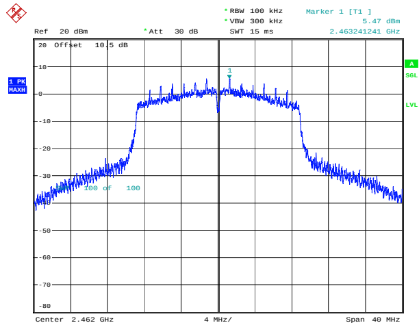
802.11n ht20_2462MHz_Reference Level
