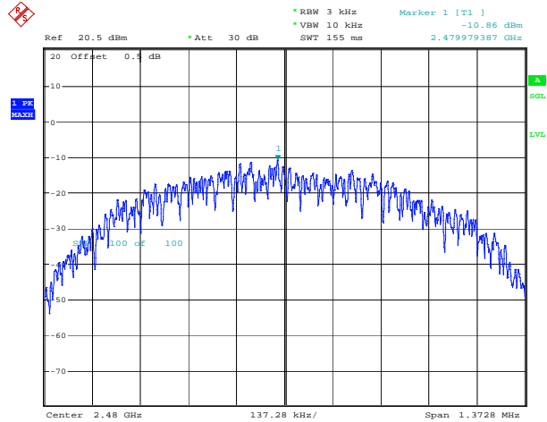
BLE_1M_High_Channel
