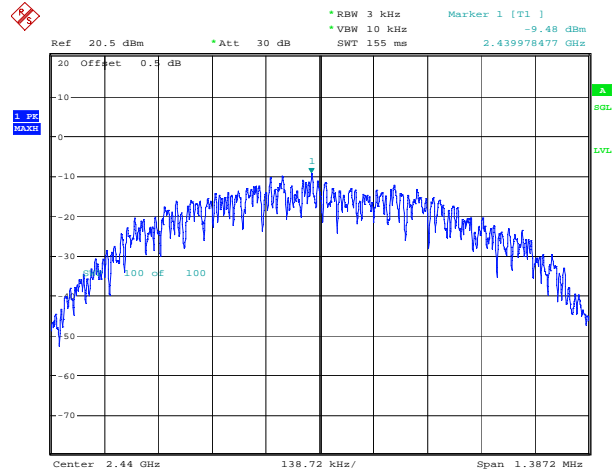
BLE_1M_Middle_Channel
