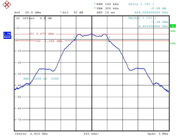
BLE_1M_Low_Channel
