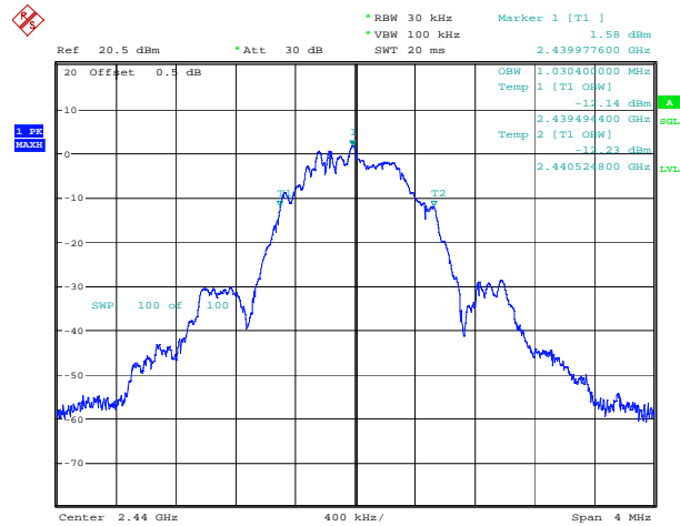
BLE_1M_Middle_Channel
