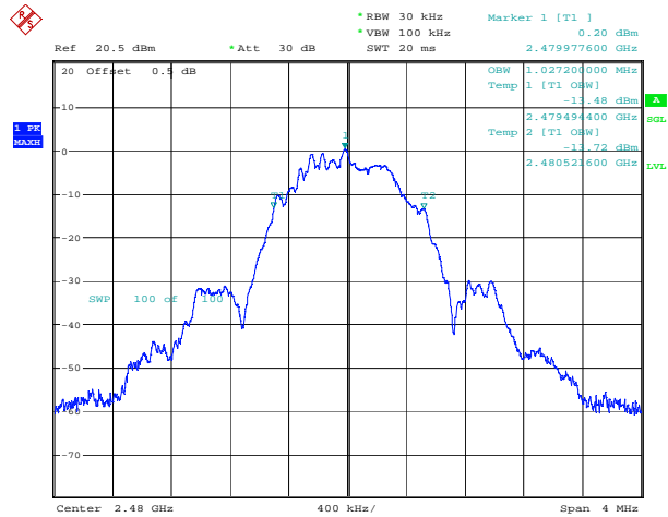
BLE_1M_High_Channel
