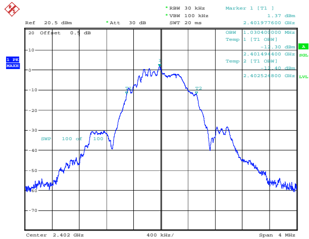
BLE_1M_Low_Channel
