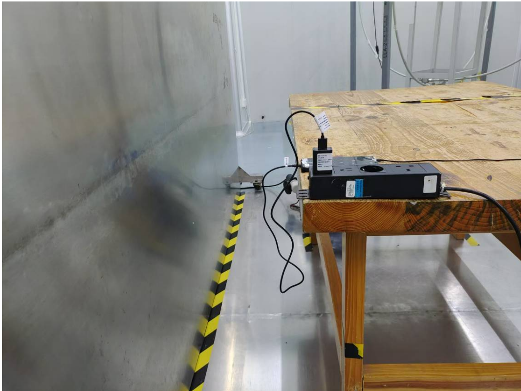
Conducted Emissions Side View Apdater 2
