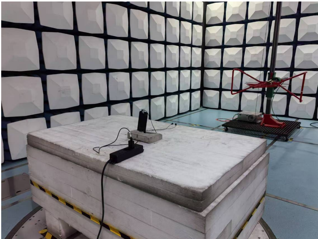
Radiated Emission 30M-1GHz View Apdater 1
