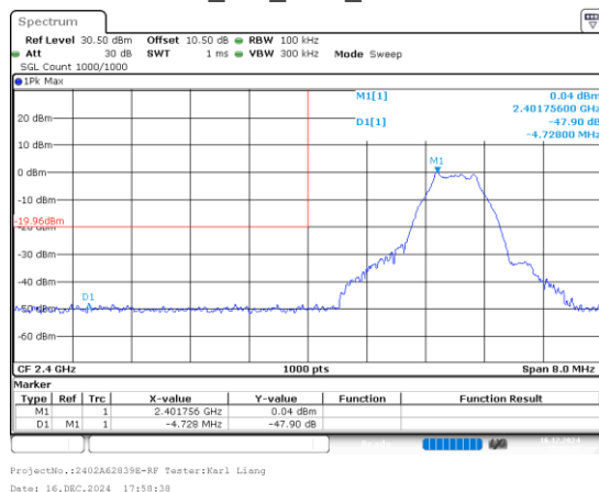
BLE_1M_Low_Channel
