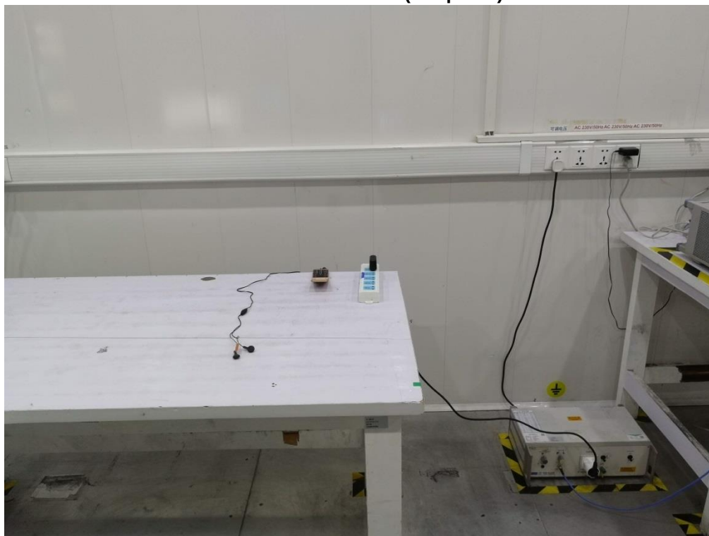
Conducted Emission(Adapter 2)
