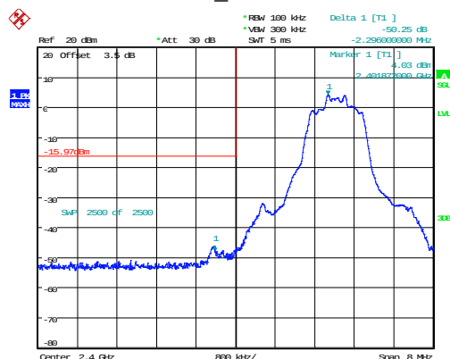
2DH1_Low 50.25dB
