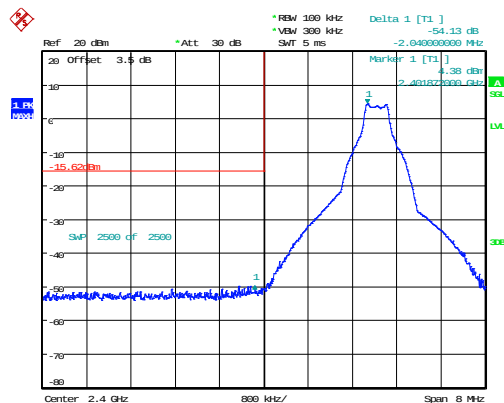
DH1_Low 54.13dB
