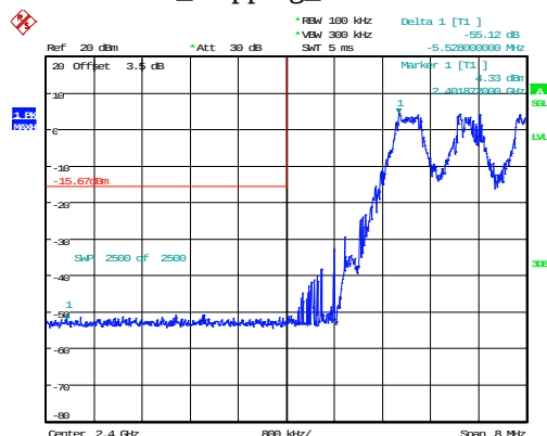
DH1_Hopping_Lower 55.12dB
