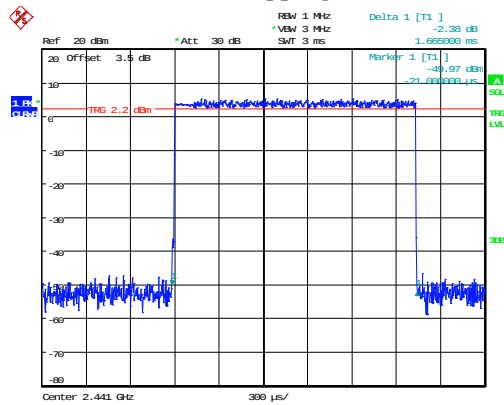
3DH3_Hopping 1.665ms
