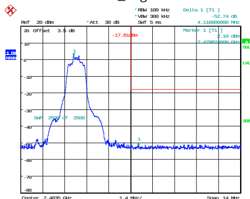
2DH1_High 52.74dB
