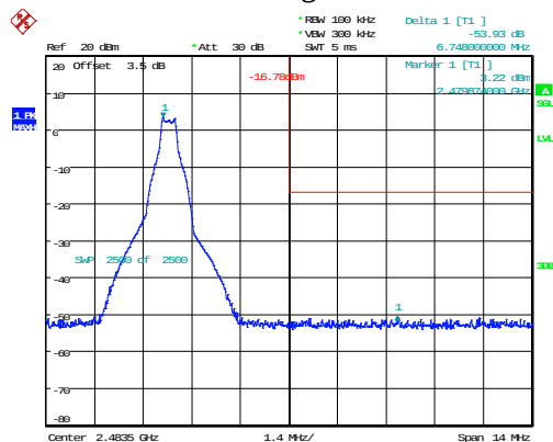
DH1_High 53.93dB
