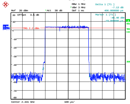
3DH1_Hopping 0.406ms
