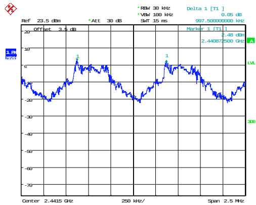
DH1_Middle 0.998MHz
