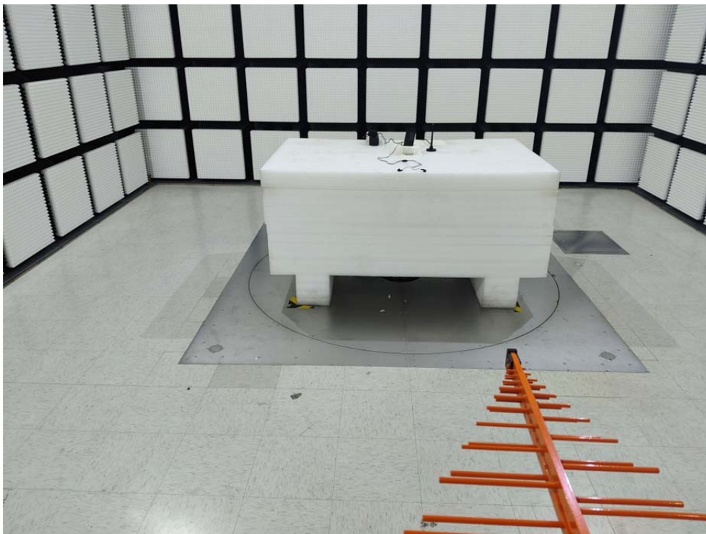
Radiated Emission 30 MHz-1 GHz View
