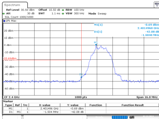
BLE_2M_Low_Channel
