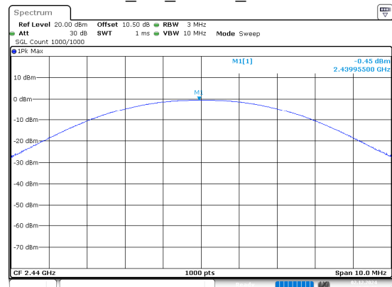
BLE_1M_Middle_Channel
