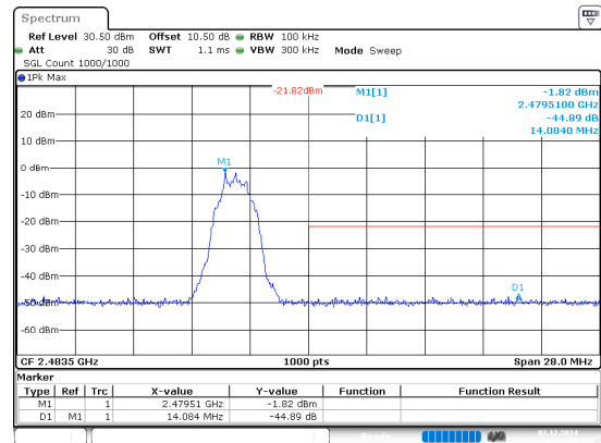
BLE_2M_High_Channel
