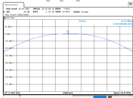
BLE_2M_Low_Channel
