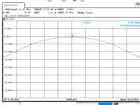
BLE_1M_High_Channel
