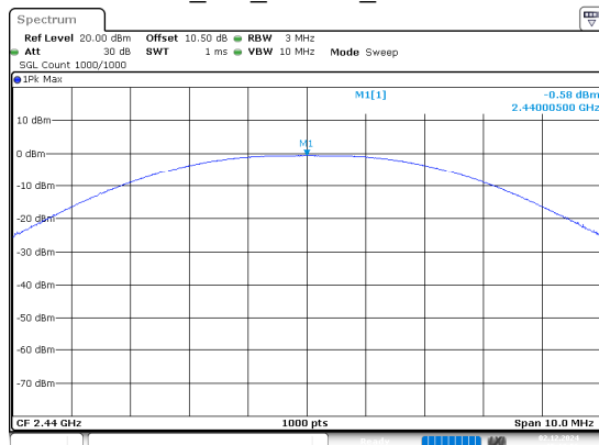
BLE_2M_Middle_Channel
