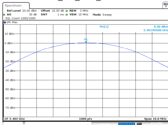
BLE_1M_Low_Channel
